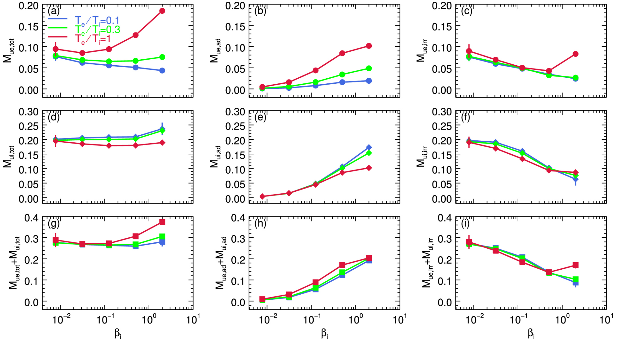
Figure 27. from Electron and Proton Heating in Transrelativistic Magnetic Reconnection null 2017 APJ 850 29 doi:10.3847/1538-4357/aa9380 https://dx.doi.org/10.3847/1538-4357/aa9380
