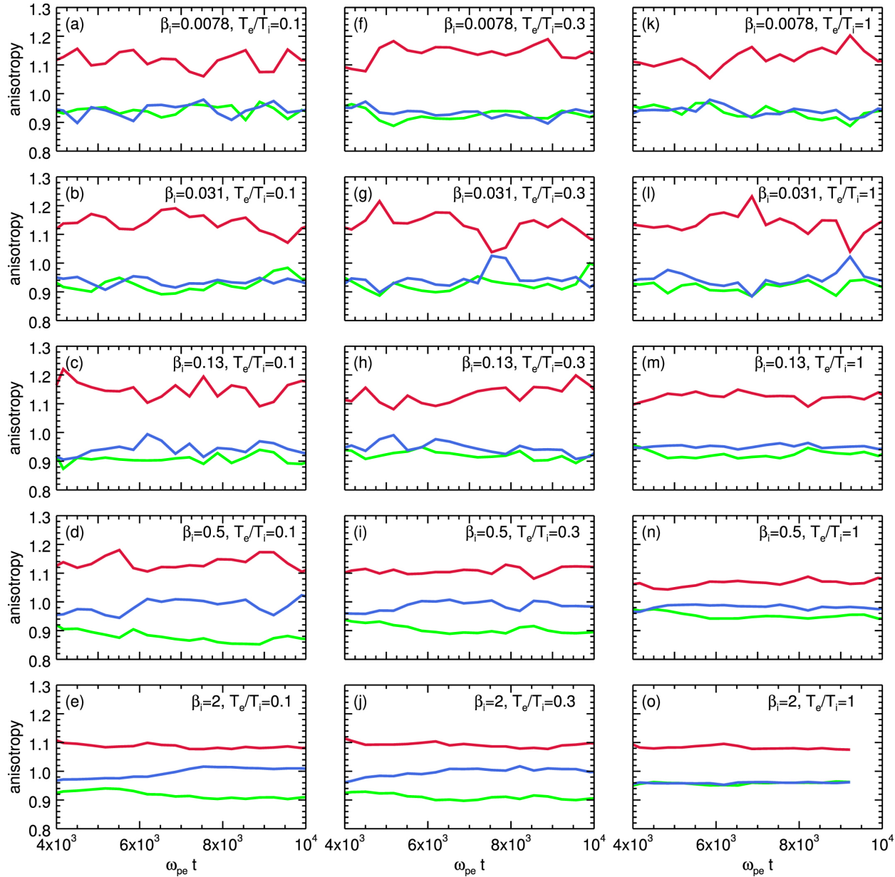
Figure 25. from Electron and Proton Heating in Transrelativistic Magnetic Reconnection null 2017 APJ 850 29 doi:10.3847/1538-4357/aa9380 https://dx.doi.org/10.3847/1538-4357/aa9380
