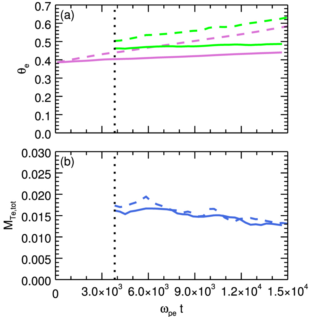
Figure 24. from Electron and Proton Heating in Transrelativistic Magnetic Reconnection null 2017 APJ 850 29 doi:10.3847/1538-4357/aa9380 https://dx.doi.org/10.3847/1538-4357/aa9380 © 2017. The American Astronomical Society. All rights reserved.
