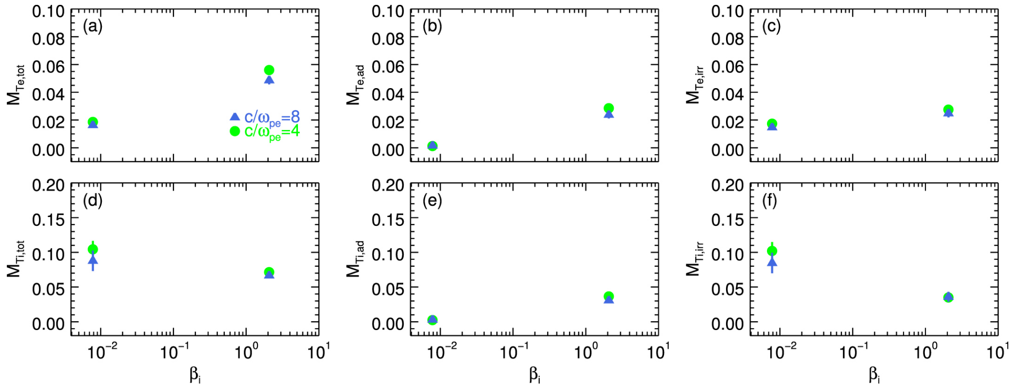
Figure 23. from Electron and Proton Heating in Transrelativistic Magnetic Reconnection null 2017 APJ 850 29 doi:10.3847/1538-4357/aa9380 https://dx.doi.org/10.3847/1538-4357/aa9380
