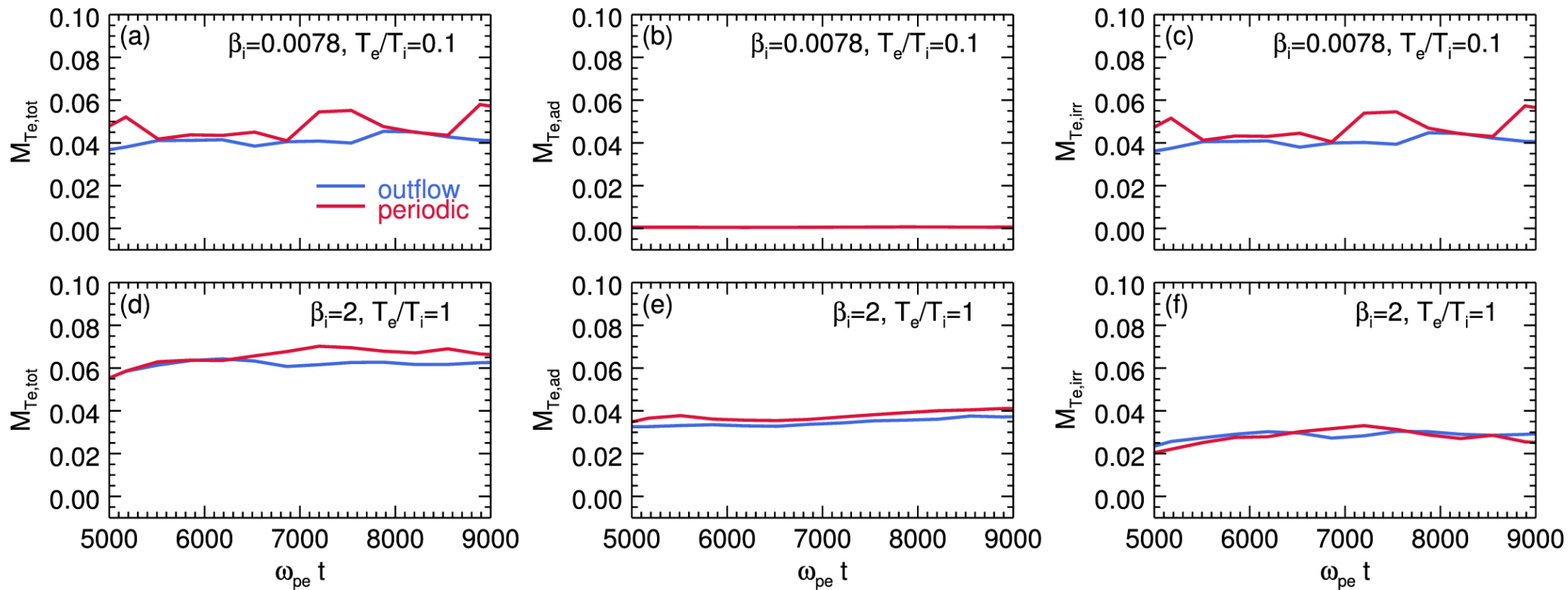
Figure 21. from Electron and Proton Heating in Transrelativistic Magnetic Reconnection null 2017 APJ 850 29 doi:10.3847/1538-4357/aa9380 https://dx.doi.org/10.3847/1538-4357/aa9380
