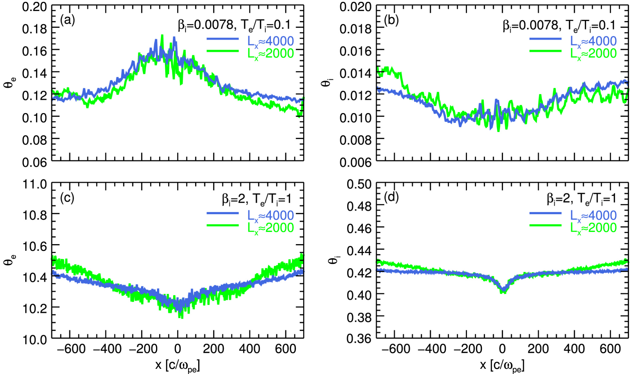
Figure 20. from Electron and Proton Heating in Transrelativistic Magnetic Reconnection null 2017 APJ 850 29 doi:10.3847/1538-4357/aa9380 https://dx.doi.org/10.3847/1538-4357/aa9380 © 2017. The American Astronomical Society. All rights reserved.
