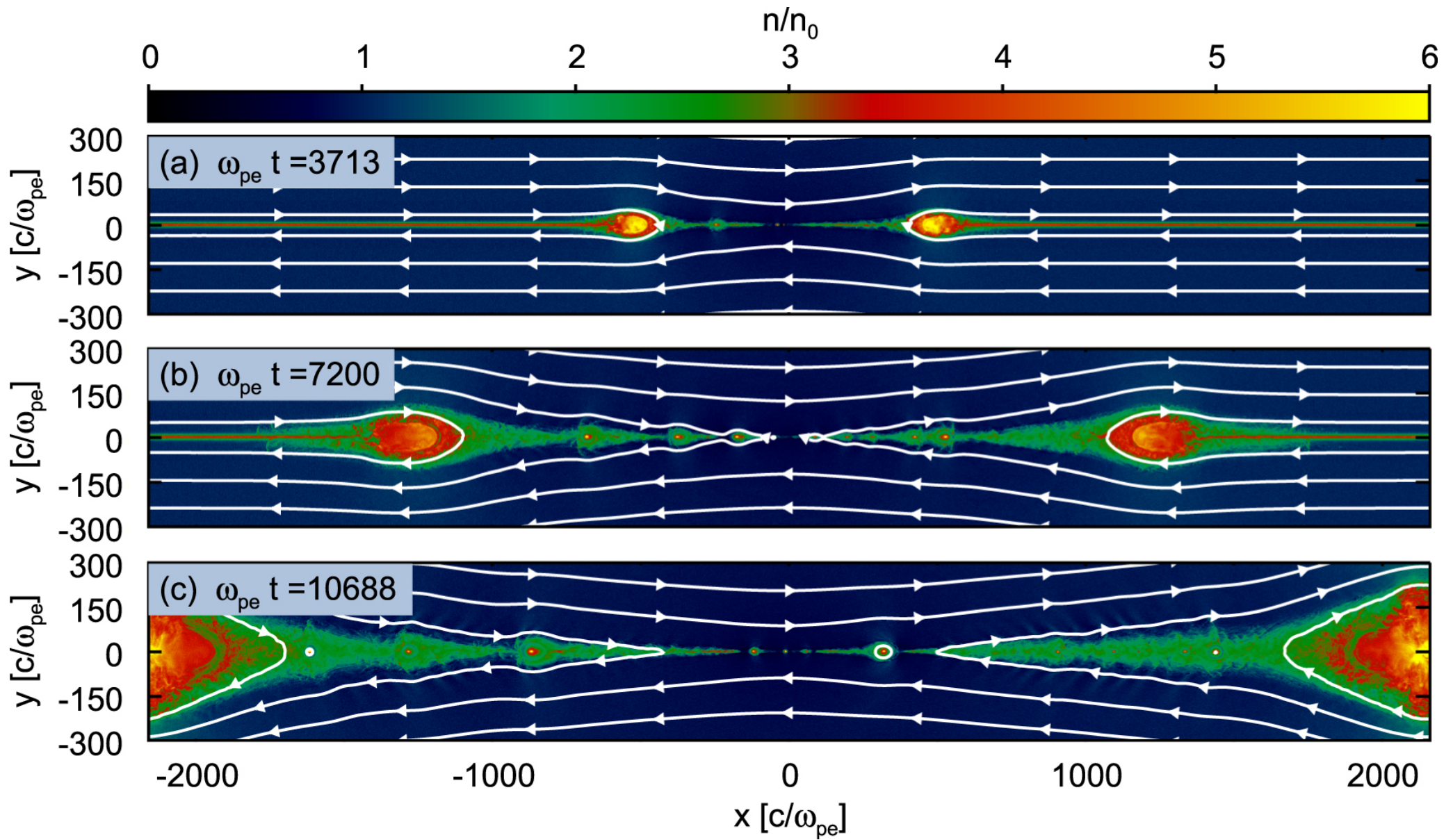
Figure 2. from Electron and Proton Heating in Transrelativistic Magnetic Reconnection null 2017 APJ 850 29 doi:10.3847/1538-4357/aa9380 https://dx.doi.org/10.3847/1538-4357/aa9380 © 2017. The American Astronomical Society. All rights reserved.
