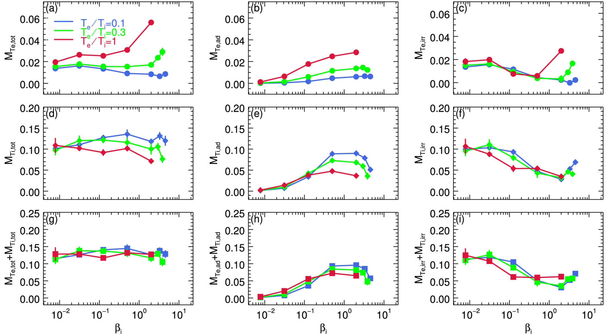
Figure 18. from Electron and Proton Heating in Transrelativistic Magnetic Reconnection null 2017 APJ 850 29 doi:10.3847/1538-4357/aa9380 https://dx.doi.org/10.3847/1538-4357/aa9380 © 2017. The American Astronomical Society. All rights reserved.
