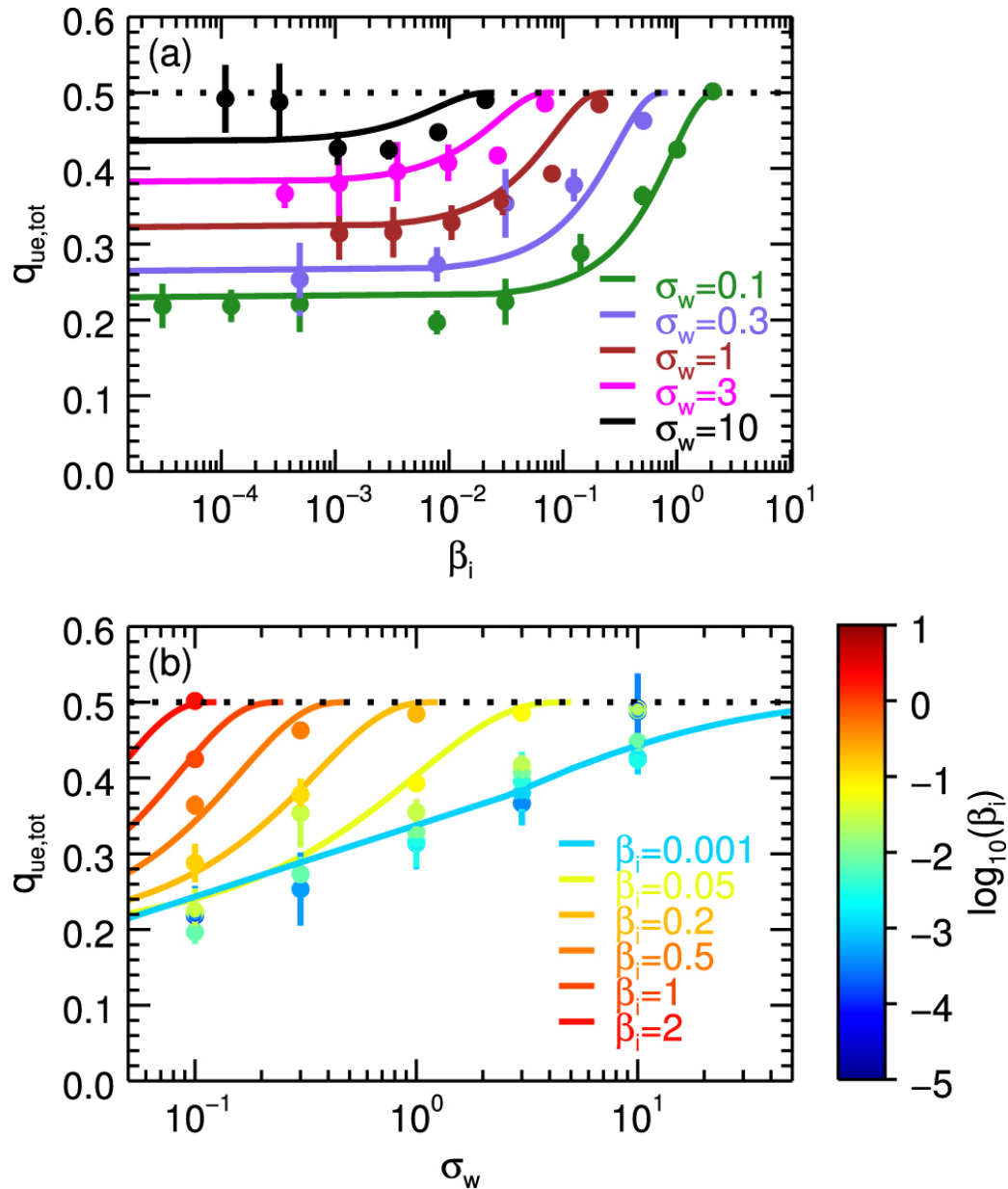
Figure 17. from Electron and Proton Heating in Transrelativistic Magnetic Reconnection null 2017 APJ 850 29 doi:10.3847/1538-4357/aa9380 https://dx.doi.org/10.3847/1538-4357/aa9380
