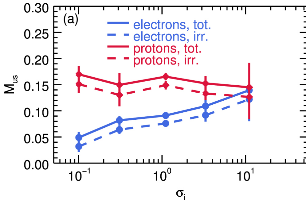
Figure 16. from Electron and Proton Heating in Transrelativistic Magnetic Reconnection null 2017 APJ 850 29 doi:10.3847/1538-4357/aa9380 https://dx.doi.org/10.3847/1538-4357/aa9380 © 2017. The American Astronomical Society. All rights reserved.
