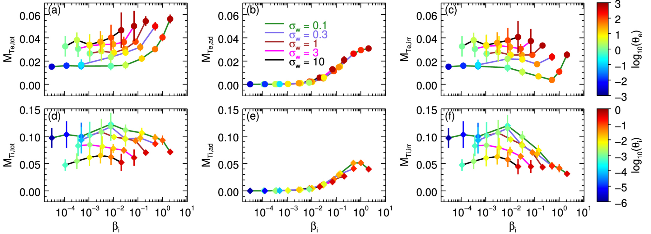
Figure 14. from Electron and Proton Heating in Transrelativistic Magnetic Reconnection null 2017 APJ 850 29 doi:10.3847/1538-4357/aa9380 https://dx.doi.org/10.3847/1538-4357/aa9380 © 2017. The American Astronomical Society. All rights reserved.
