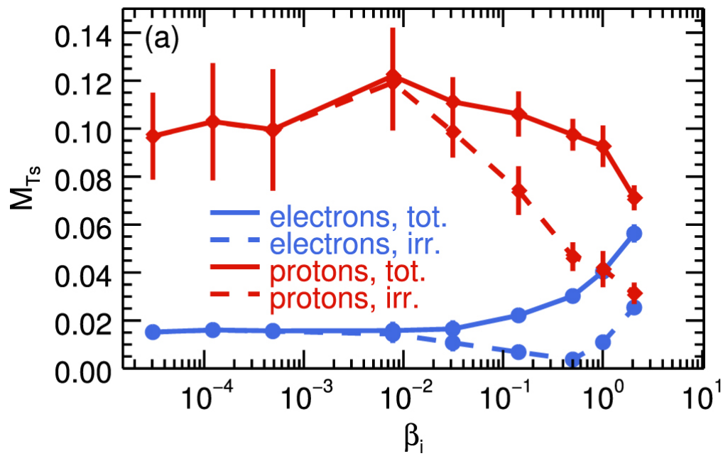
Figure 13. from Electron and Proton Heating in Transrelativistic Magnetic Reconnection null 2017 APJ 850 29 doi:10.3847/1538-4357/aa9380 https://dx.doi.org/10.3847/1538-4357/aa9380 © 2017. The American Astronomical Society. All rights reserved.
