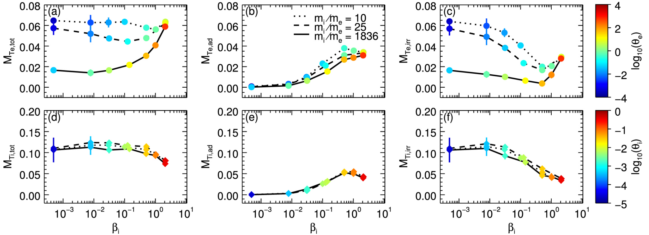
Figure 12. from Electron and Proton Heating in Transrelativistic Magnetic Reconnection null 2017 APJ 850 29 doi:10.3847/1538-4357/aa9380 https://dx.doi.org/10.3847/1538-4357/aa9380
