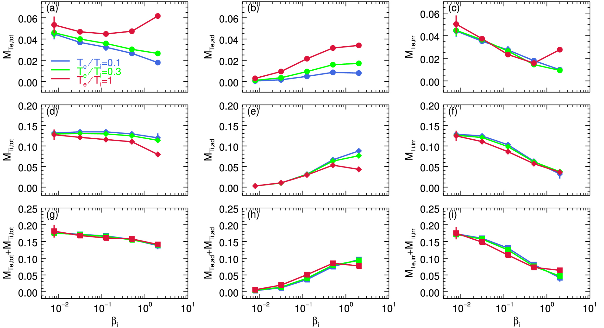
Figure 11. from Electron and Proton Heating in Transrelativistic Magnetic Reconnection null 2017 APJ 850 29 doi:10.3847/1538-4357/aa9380 https://dx.doi.org/10.3847/1538-4357/aa9380
