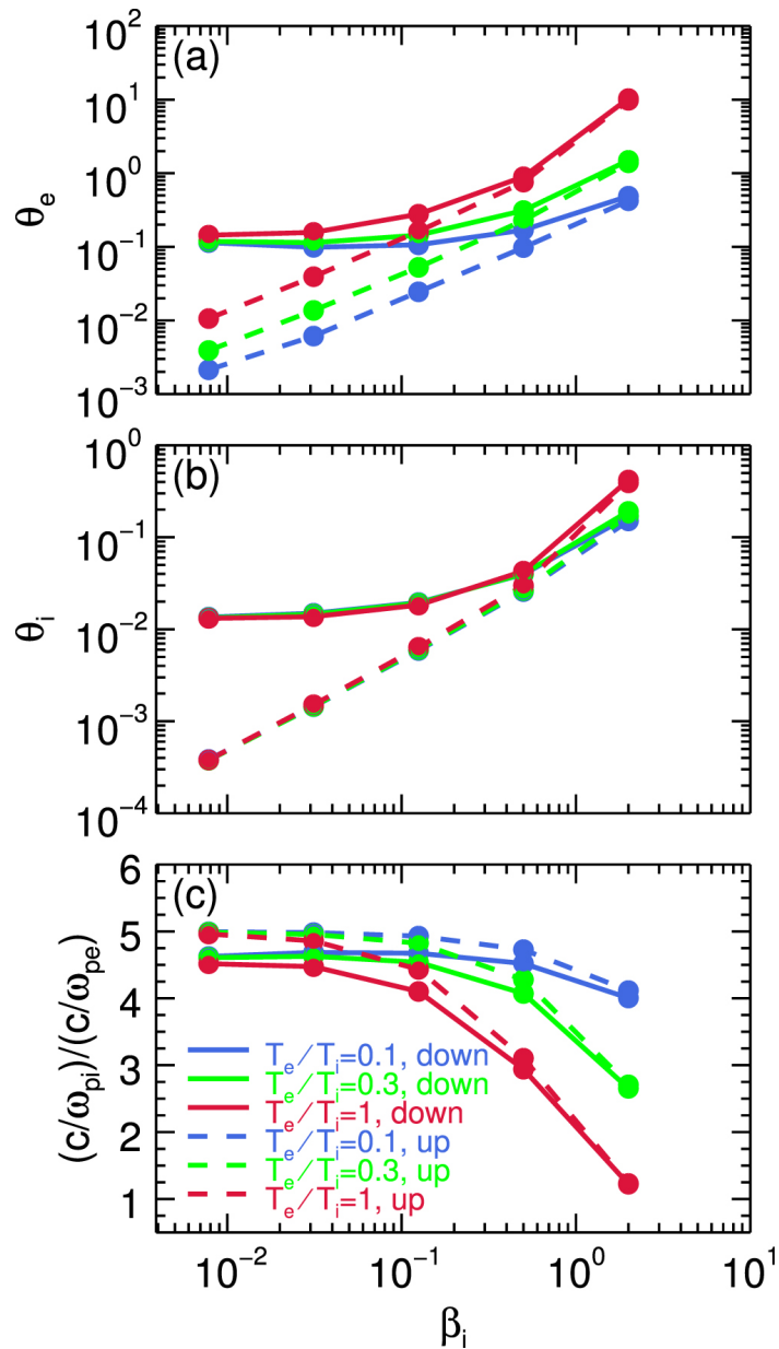
Figure 10. from Electron and Proton Heating in Transrelativistic Magnetic Reconnection null 2017 APJ 850 29 doi:10.3847/1538-4357/aa9380 https://dx.doi.org/10.3847/1538-4357/aa9380 © 2017. The American Astronomical Society. All rights reserved.
