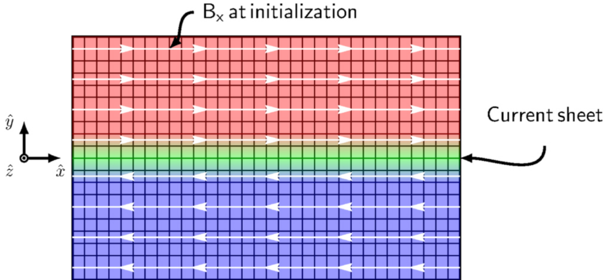
Figure 1. from Electron and Proton Heating in Transrelativistic Magnetic Reconnection null 2017 APJ 850 29 doi:10.3847/1538-4357/aa9380 https://dx.doi.org/10.3847/1538-4357/aa9380 © 2017. The American Astronomical Society. All rights reserved.
