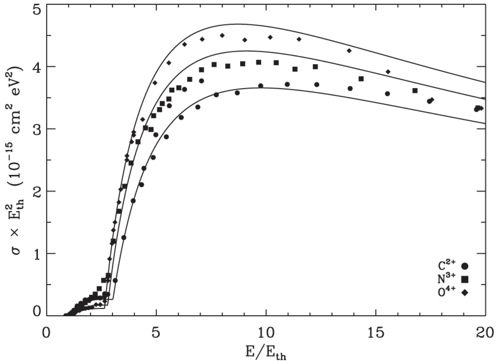
Figure 3. from Electron-impact Multiple-ionization Cross Sections for Atoms and Ions of Helium through Zinc null 2017 APJ 850 122 doi:10.3847/1538-4357/aa9276 https://dx.doi.org/10.3847/1538-4357/aa9276 © 2017. The American Astronomical Society. All rights reserved.
