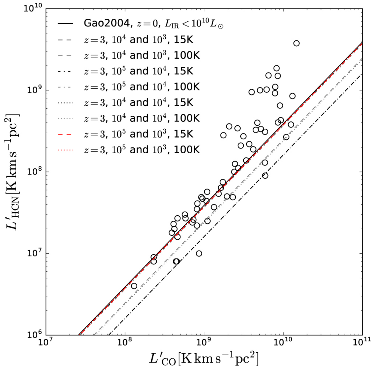
Figure 7. from The Role of the CMB in Redshift Related Departures from the Gao–Solomon Relation null 2017 APJ 849 37 doi:10.3847/1538-4357/aa8e4d https://dx.doi.org/10.3847/1538-4357/aa8e4d © 2017. The American Astronomical Society. All rights reserved.
