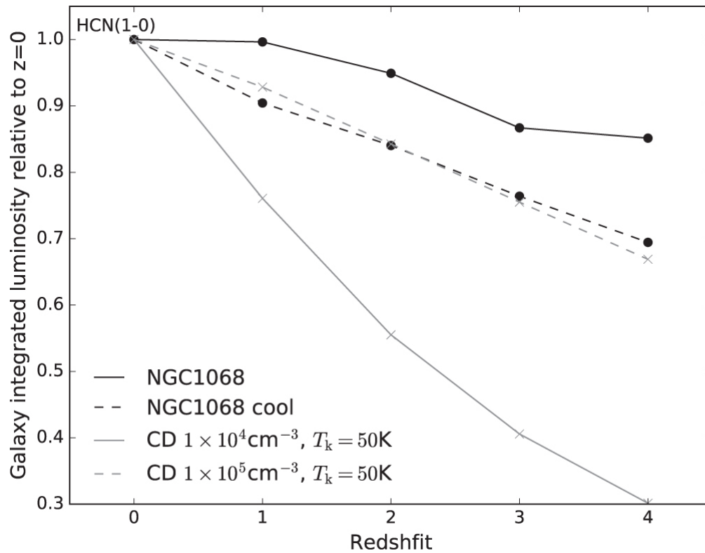
Figure 5. from The Role of the CMB in Redshift Related Departures from the Gao–Solomon Relation null 2017 APJ 849 37 doi:10.3847/1538-4357/aa8e4d https://dx.doi.org/10.3847/1538-4357/aa8e4d © 2017. The American Astronomical Society. All rights reserved.
