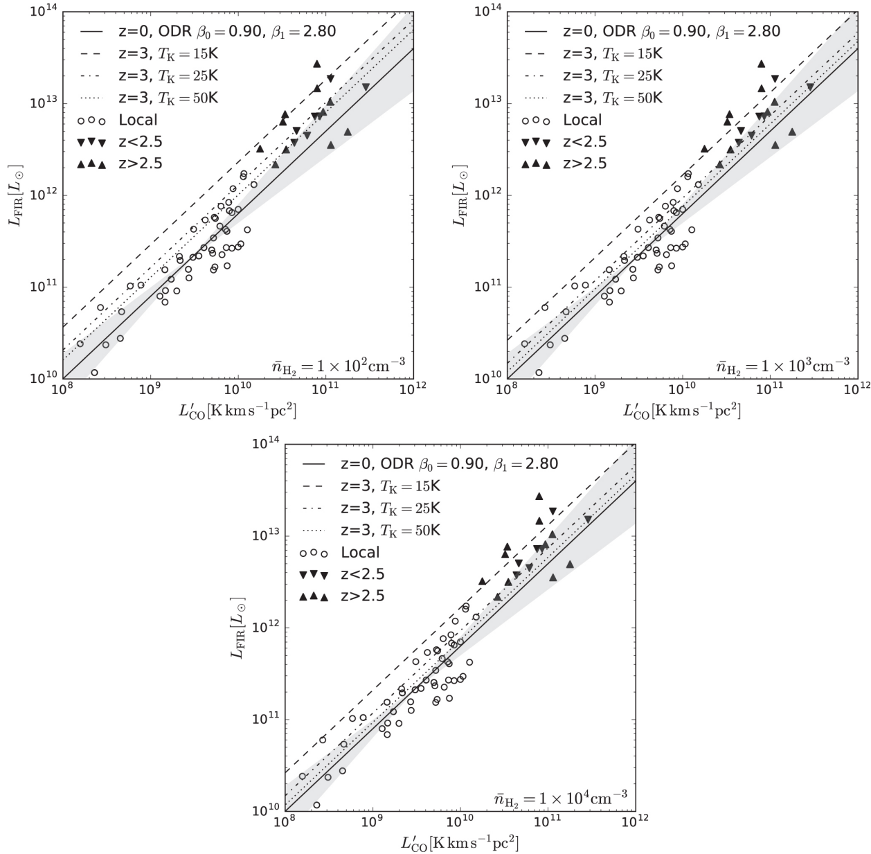
Figure 4. from The Role of the CMB in Redshift Related Departures from the Gao–Solomon Relation null 2017 APJ 849 37 doi:10.3847/1538-4357/aa8e4d https://dx.doi.org/10.3847/1538-4357/aa8e4d © 2017. The American Astronomical Society. All rights reserved.
