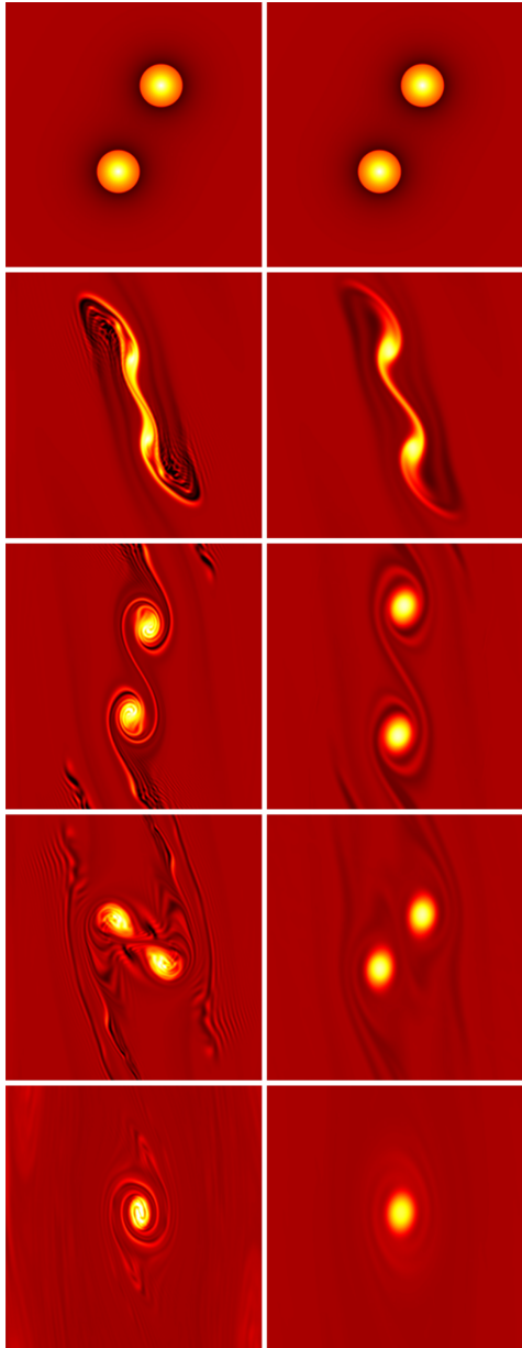
Figure 8. from A Vorticity-preserving Hydrodynamical Scheme for Modeling Accretion Disk Flows null 2017 APJ 848 54 doi:10.3847/1538-4357/aa8e45 https://dx.doi.org/10.3847/1538-4357/aa8e45 © 2017. The American Astronomical Society. All rights reserved.
