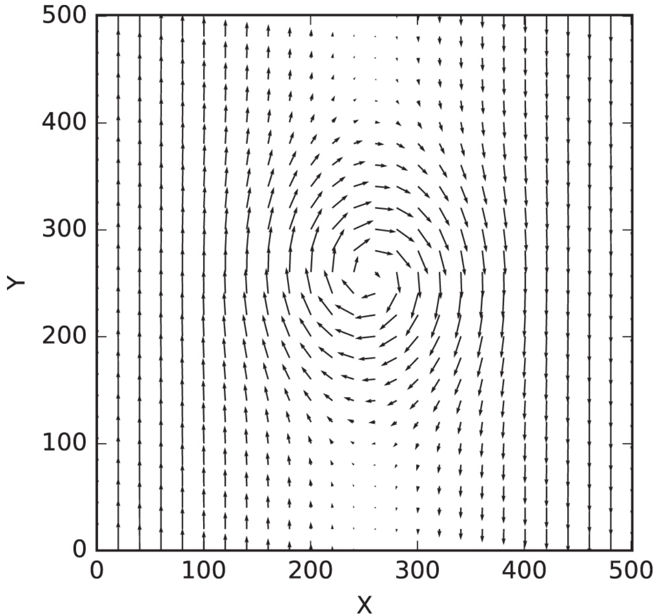
Figure 6. from A Vorticity-preserving Hydrodynamical Scheme for Modeling Accretion Disk Flows null 2017 APJ 848 54 doi:10.3847/1538-4357/aa8e45 https://dx.doi.org/10.3847/1538-4357/aa8e45 © 2017. The American Astronomical Society. All rights reserved.
