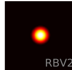
Figure 2. from A Vorticity-preserving Hydrodynamical Scheme for Modeling Accretion Disk Flows null 2017 APJ 848 54 doi:10.3847/1538-4357/aa8e45 https://dx.doi.org/10.3847/1538-4357/aa8e45 © 2017. The American Astronomical Society. All rights reserved.
