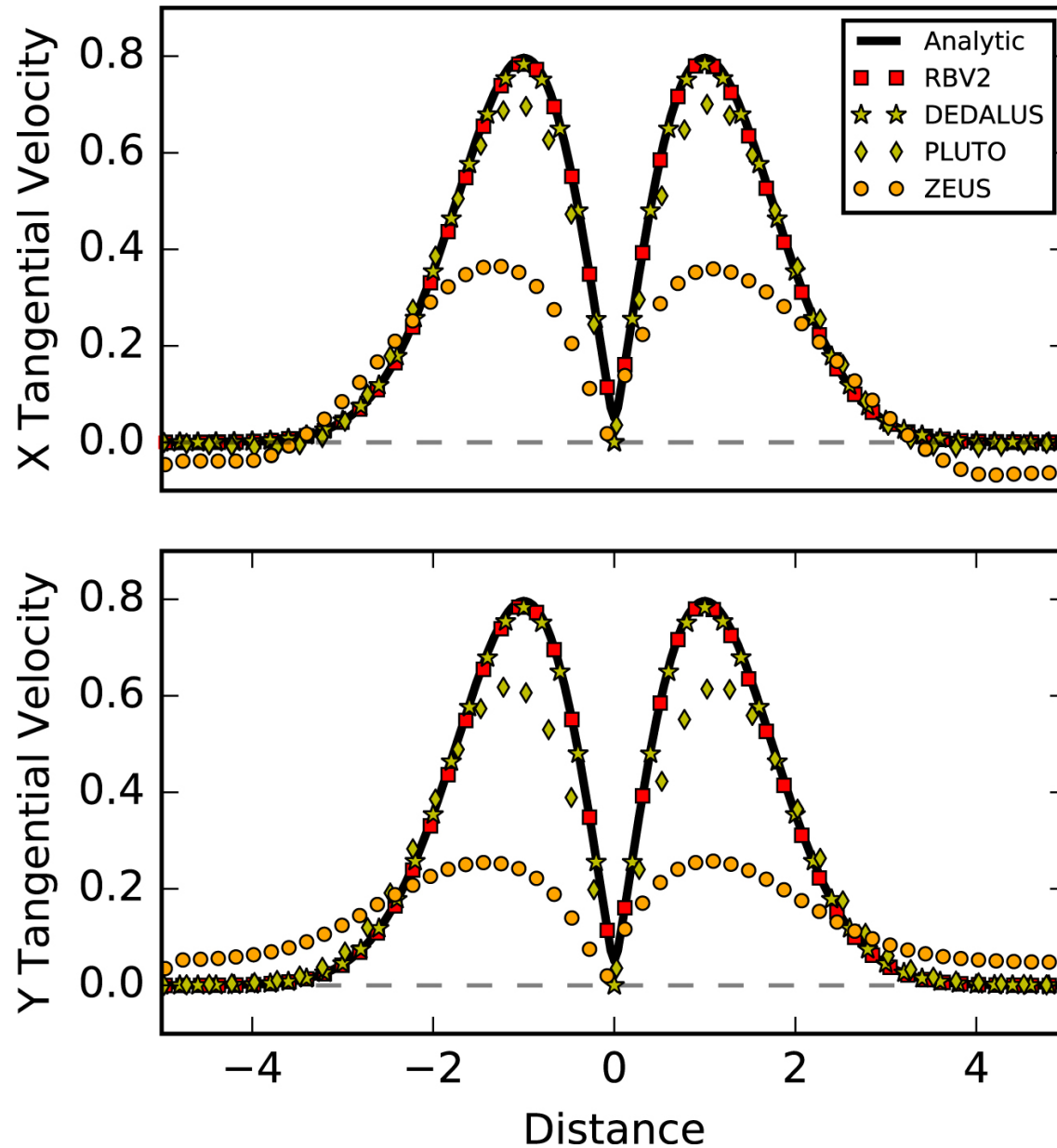
Figure 2. from A Vorticity-preserving Hydrodynamical Scheme for Modeling Accretion Disk Flows null 2017 APJ 848 54 doi:10.3847/1538-4357/aa8e45 https://dx.doi.org/10.3847/1538-4357/aa8e45 © 2017. The American Astronomical Society. All rights reserved.
