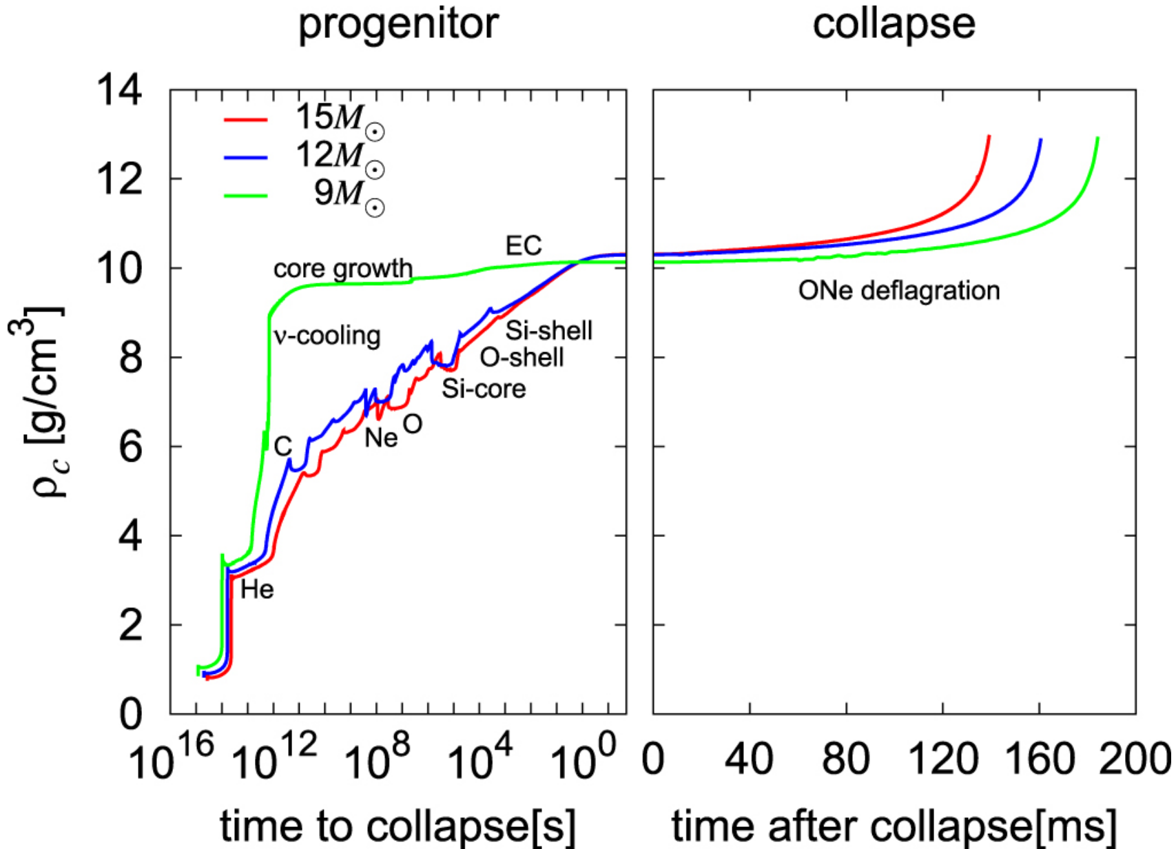
Figure 2. from Neutrino Emissions in All Flavors up to the Pre-bounce of Massive Stars and the Possibility of Their Detections null 2017 APJ 848 48 doi:10.3847/1538-4357/aa8b72 https://dx.doi.org/10.3847/1538-4357/aa8b72 © 2017. The American Astronomical Society. All rights reserved.
