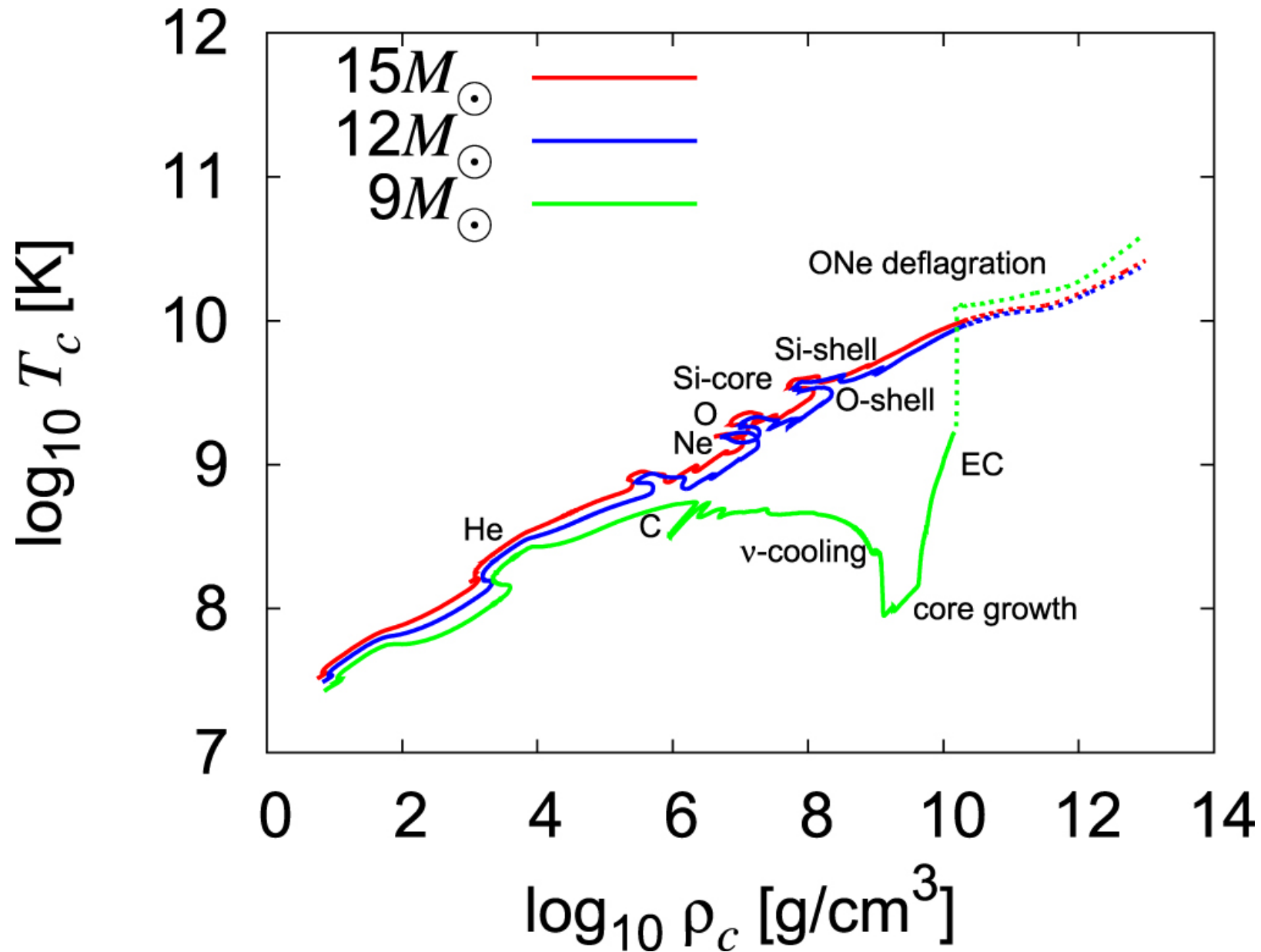
Figure 1. from Neutrino Emissions in All Flavors up to the Pre-bounce of Massive Stars and the Possibility of Their Detections null 2017 APJ 848 48 doi:10.3847/1538-4357/aa8b72 https://dx.doi.org/10.3847/1538-4357/aa8b72 © 2017. The American Astronomical Society. All rights reserved.
