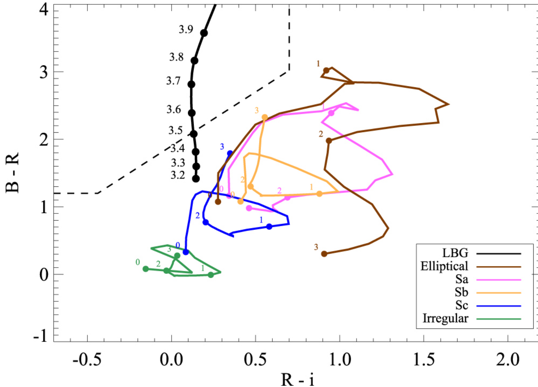
Figure 6. from Strong Clustering of Lyman Break Galaxies around Luminous Quasars at Z \sim 4 null 2017 APJ 848 7 doi:10.3847/1538-4357/aa8b69 https://dx.doi.org/10.3847/1538-4357/aa8b69 © 2017. The American Astronomical Society. All rights reserved.
