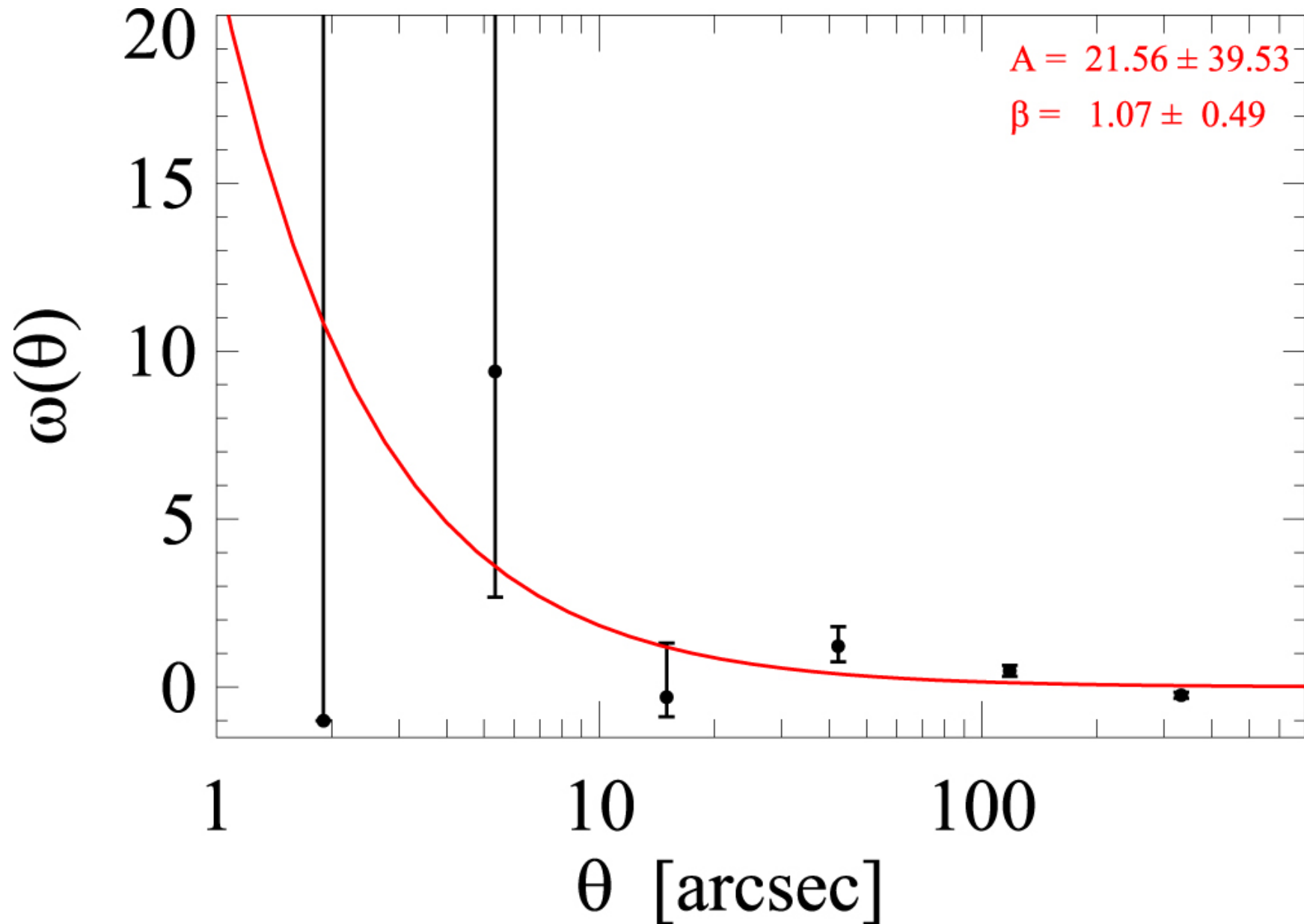
Figure 18. from Strong Clustering of Lyman Break Galaxies around Luminous Quasars at Z \sim 4 null 2017 APJ 848 7 doi:10.3847/1538-4357/aa8b69 https://dx.doi.org/10.3847/1538-4357/aa8b69 © 2017. The American Astronomical Society. All rights reserved.
