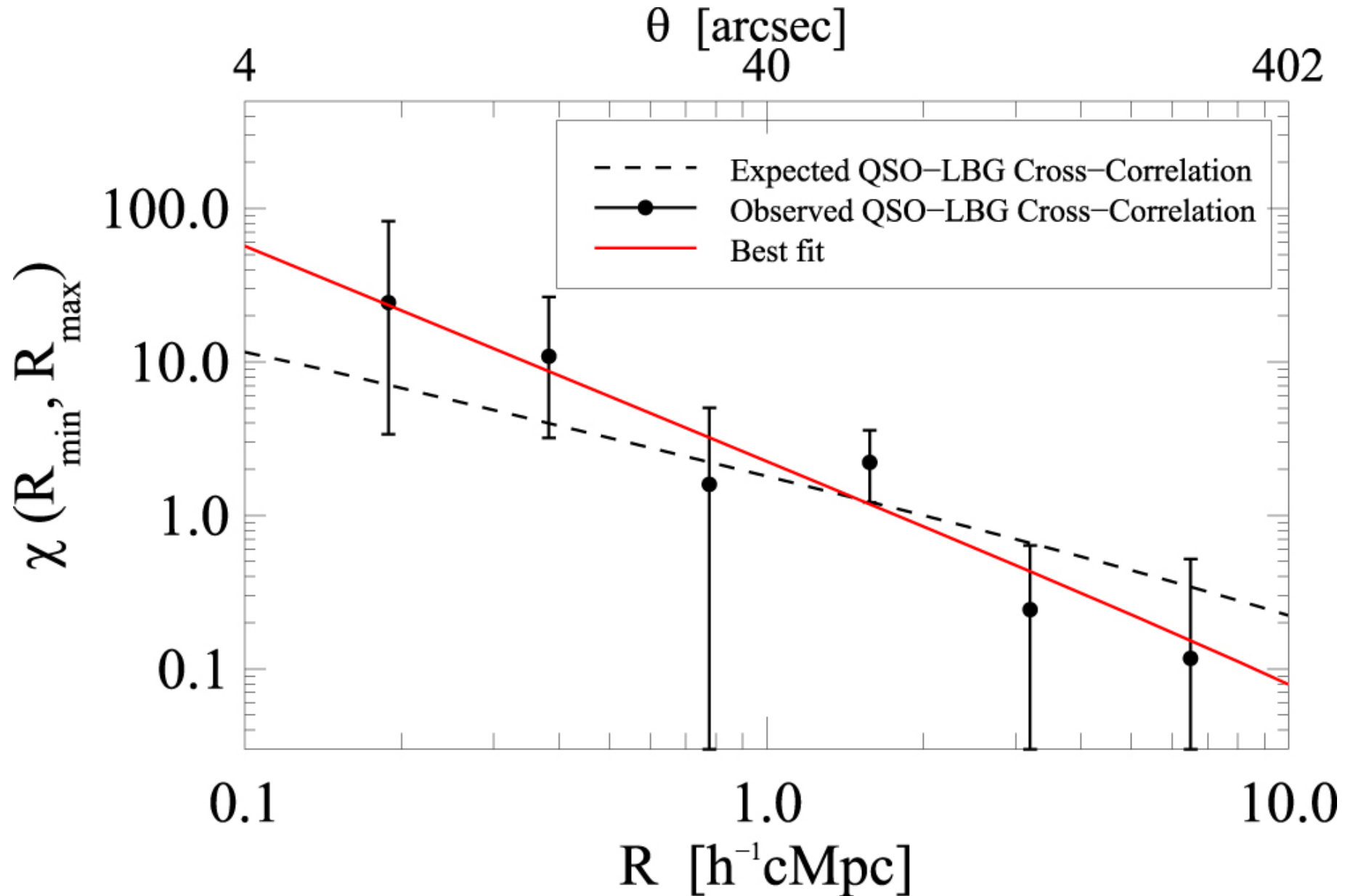
Figure 14. from Strong Clustering of Lyman Break Galaxies around Luminous Quasars at Z \sim 4 null 2017 APJ 848 7 doi:10.3847/1538-4357/aa8b69 https://dx.doi.org/10.3847/1538-4357/aa8b69 © 2017. The American Astronomical Society. All rights reserved.
