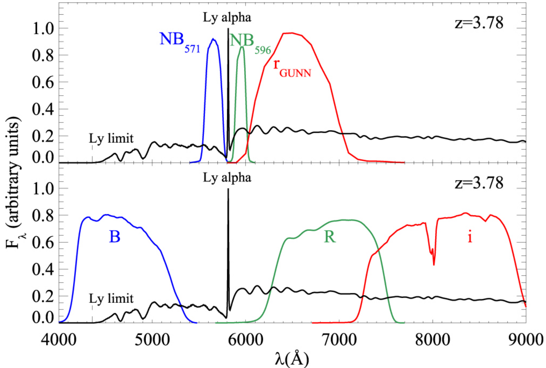
Figure 1. from Strong Clustering of Lyman Break Galaxies around Luminous Quasars at Z \sim 4 null 2017 APJ 848 7 doi:10.3847/1538-4357/aa8b69 https://dx.doi.org/10.3847/1538-4357/aa8b69 © 2017. The American Astronomical Society. All rights reserved.
