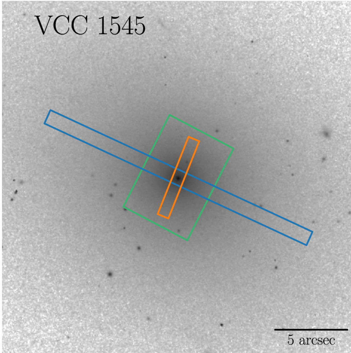
Figure 6. from Virgo Redux: The Masses and Stellar Content of Nuclei in Early-type Galaxies from Multiband Photometry and Spectroscopy null 2017 APJ 849 55 doi:10.3847/1538-4357/aa8a78 https://dx.doi.org/10.3847/1538-4357/aa8a78 © 2017. The American Astronomical Society. All rights reserved.
