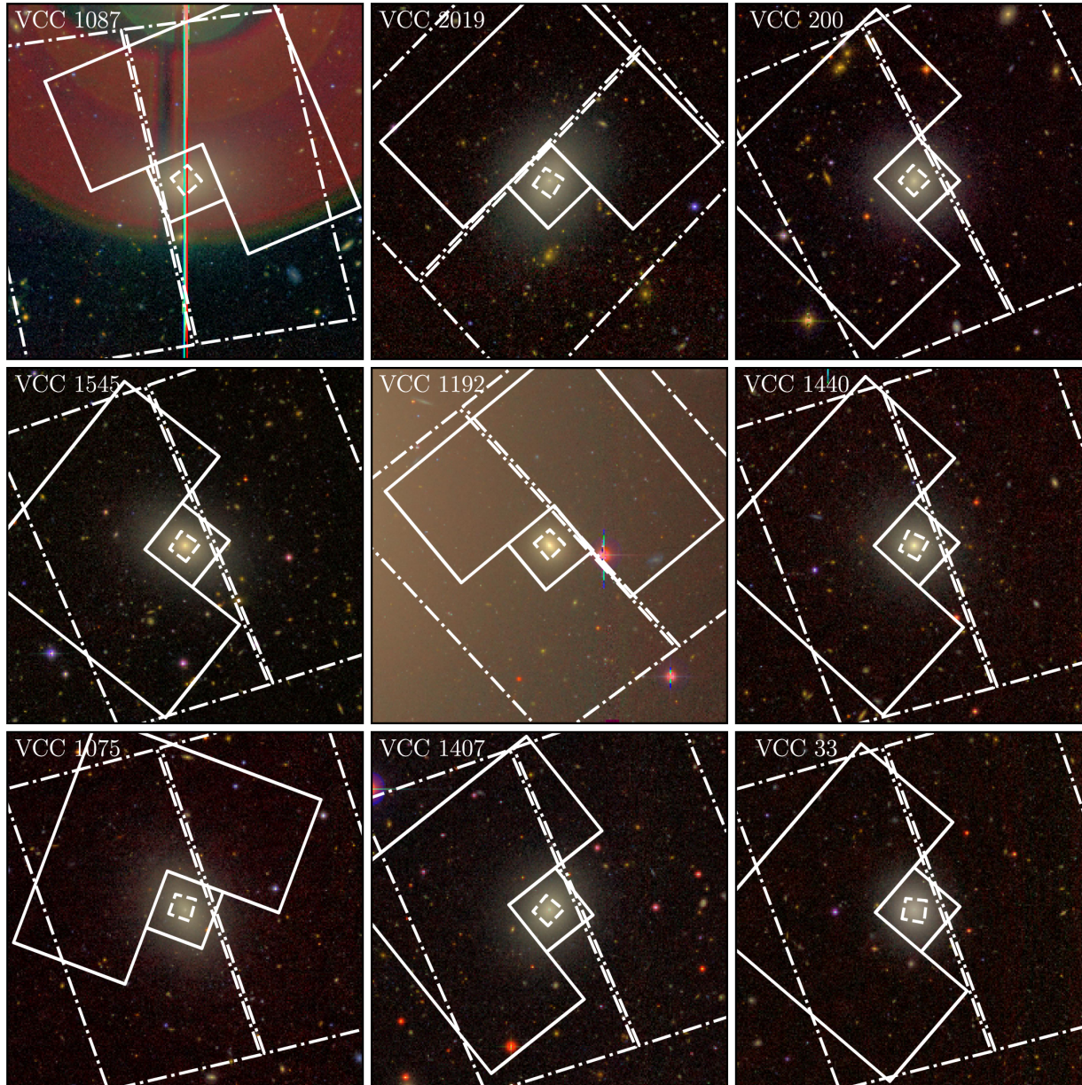
Figure 1. from Virgo Redux: The Masses and Stellar Content of Nuclei in Early-type Galaxies from Multiband Photometry and Spectroscopy null 2017 APJ 849 55 doi:10.3847/1538-4357/aa8a78 https://dx.doi.org/10.3847/1538-4357/aa8a78 © 2017. The American Astronomical Society. All rights reserved.
