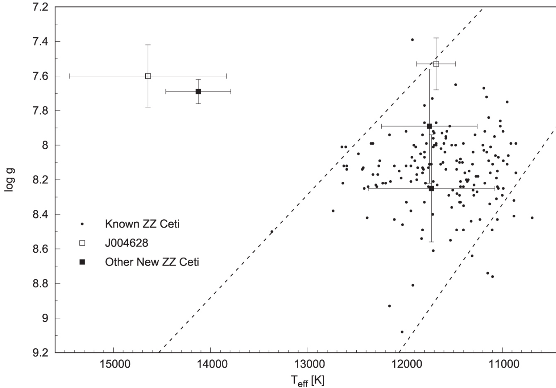
Figure 8. from New ZZ Ceti Stars from the LAMOST Survey null 2017 APJ 847 34 doi:10.3847/1538-4357/aa88a8 https://dx.doi.org/10.3847/1538-4357/aa88a8 © 2017. The American Astronomical Society. All rights reserved.
