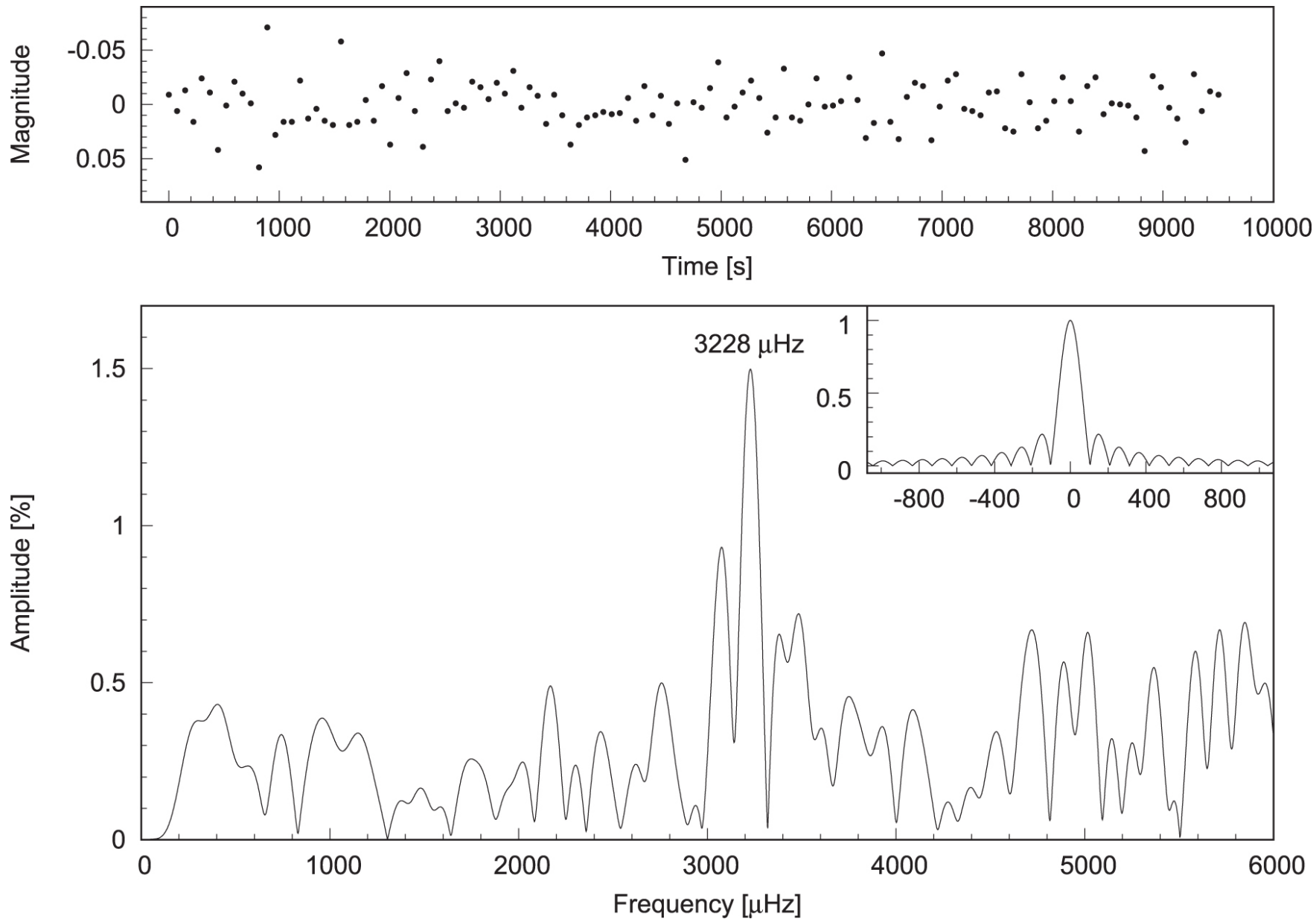
Figure 5. from New ZZ Ceti Stars from the LAMOST Survey null 2017 APJ 847 34 doi:10.3847/1538-4357/aa88a8 https://dx.doi.org/10.3847/1538-4357/aa88a8 © 2017. The American Astronomical Society. All rights reserved.
