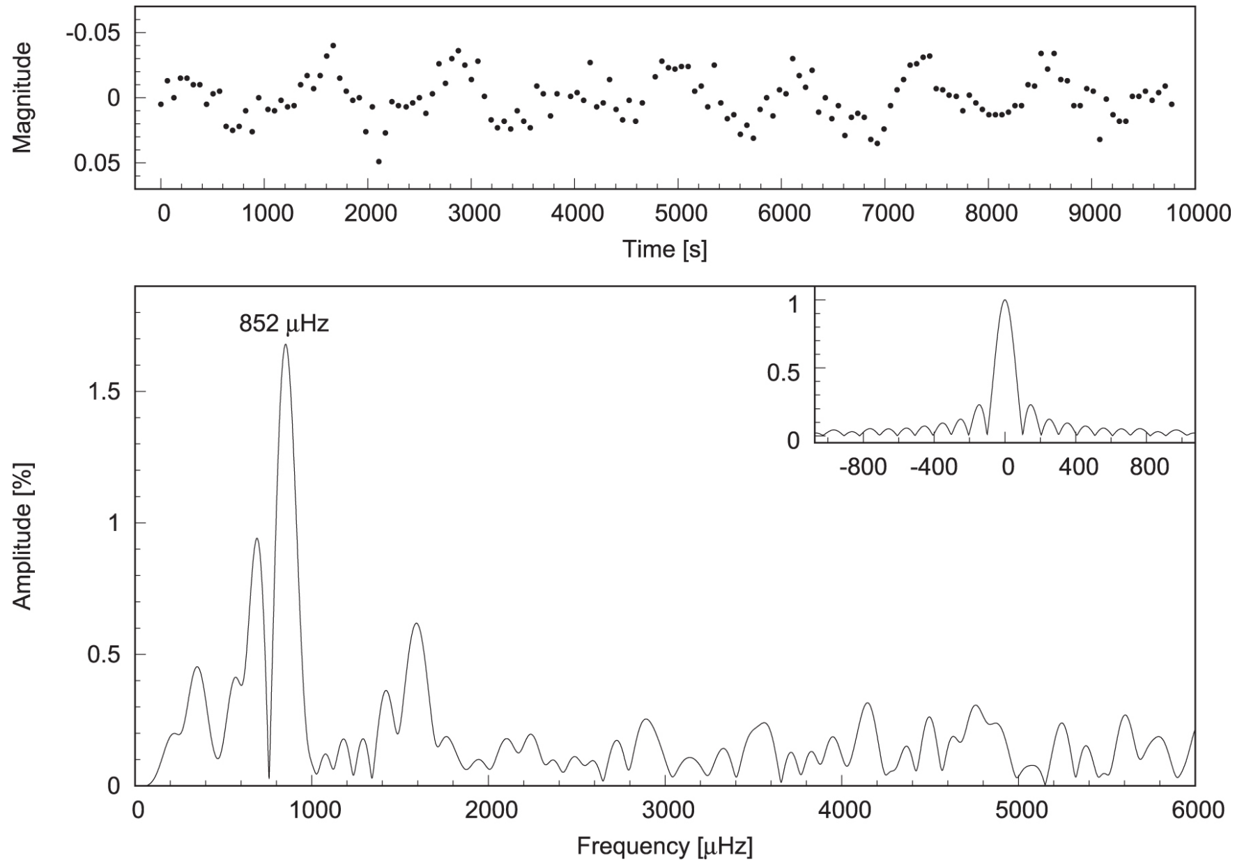
Figure 4. from New ZZ Ceti Stars from the LAMOST Survey null 2017 APJ 847 34 doi:10.3847/1538-4357/aa88a8 https://dx.doi.org/10.3847/1538-4357/aa88a8 © 2017. The American Astronomical Society. All rights reserved.
