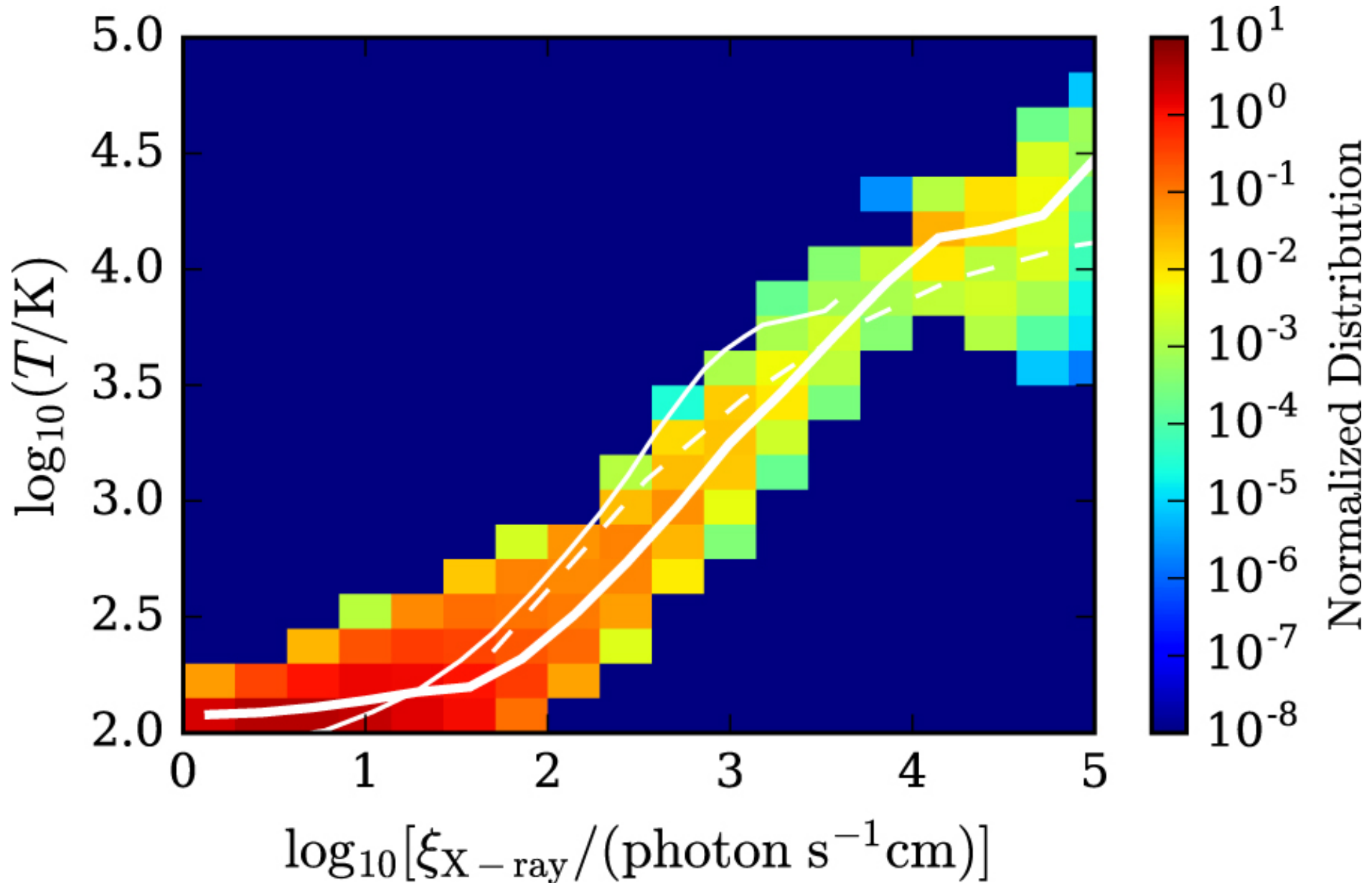
Figure 9. from Hydrodynamic Photoevaporation of Protoplanetary Disks with Consistent Thermochemistry null 2017 APJ 847 11 doi:10.3847/1538-4357/aa8726 https://dx.doi.org/10.3847/1538-4357/aa8726 © 2017. The American Astronomical Society. All rights reserved.
