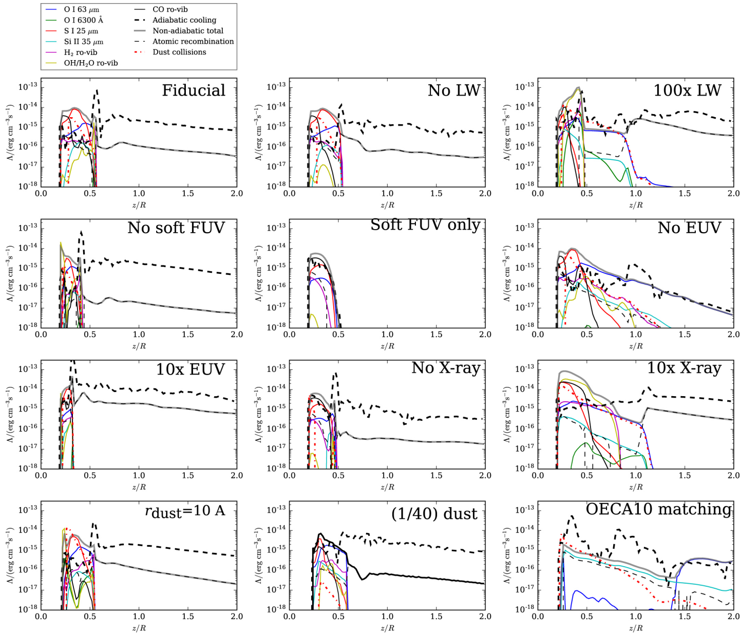
Figure 7. from Hydrodynamic Photoevaporation of Protoplanetary Disks with Consistent Thermochemistry null 2017 APJ 847 11 doi:10.3847/1538-4357/aa8726 https://dx.doi.org/10.3847/1538-4357/aa8726 © 2017. The American Astronomical Society. All rights reserved.
