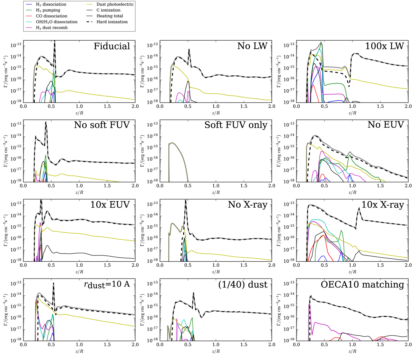
Figure 6. from Hydrodynamic Photoevaporation of Protoplanetary Disks with Consistent Thermochemistry null 2017 APJ 847 11 doi:10.3847/1538-4357/aa8726 https://dx.doi.org/10.3847/1538-4357/aa8726 © 2017. The American Astronomical Society. All rights reserved.
