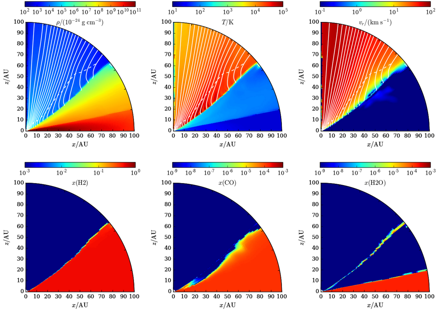
Figure 1. from Hydrodynamic Photoevaporation of Protoplanetary Disks with Consistent Thermochemistry null 2017 APJ 847 11 doi:10.3847/1538-4357/aa8726 https://dx.doi.org/10.3847/1538-4357/aa8726 © 2017. The American Astronomical Society. All rights reserved.
