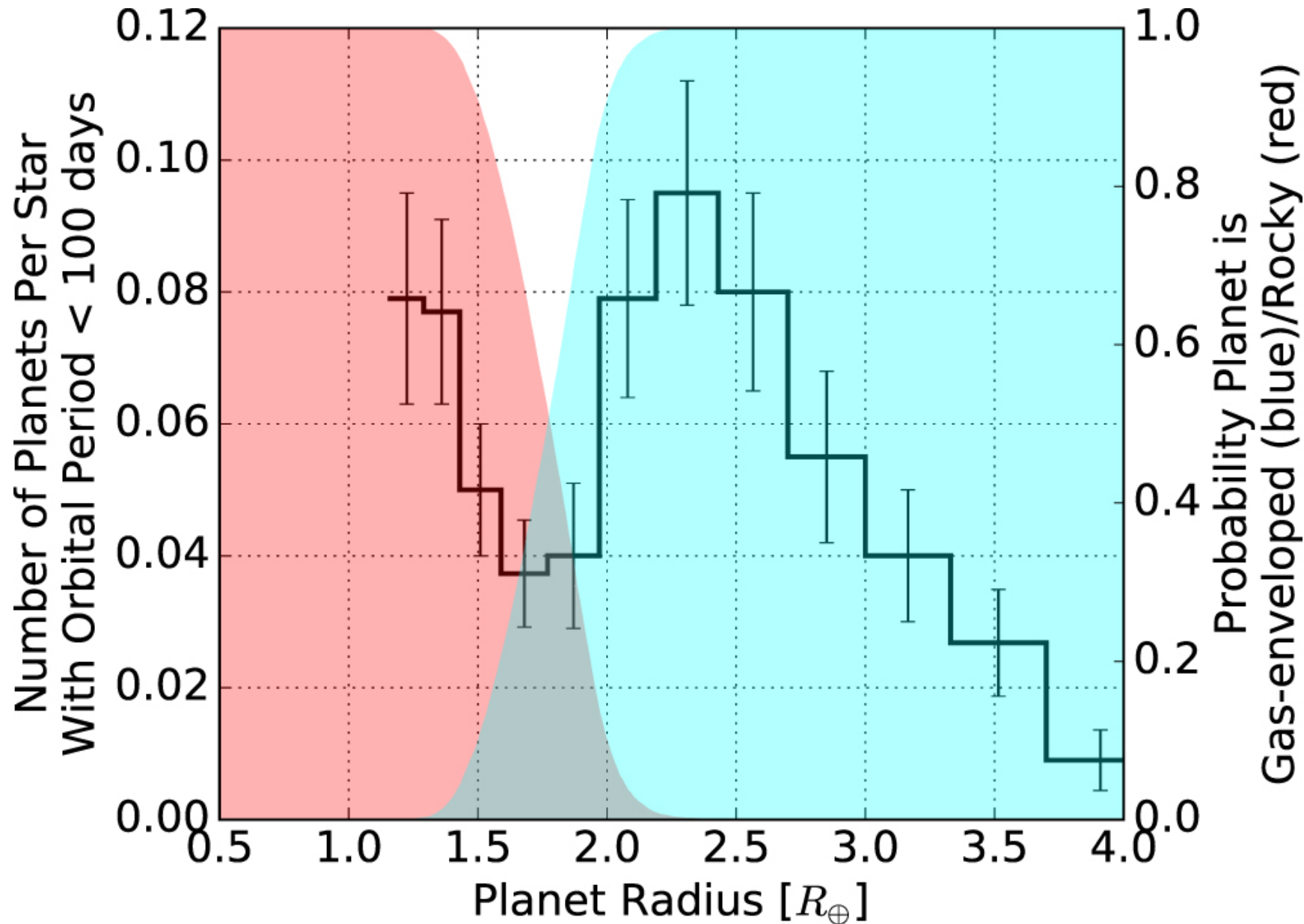
Figure 5. from Rocky Worlds Limited to 1.8 Earth Radii by Atmospheric Escape during a Star's Extreme UV Saturation null 2017 APJ 845 130 doi:10.3847/1538-4357/aa8137 https://dx.doi.org/10.3847/1538-4357/aa8137 © 2017. The American Astronomical Society. All rights reserved.
