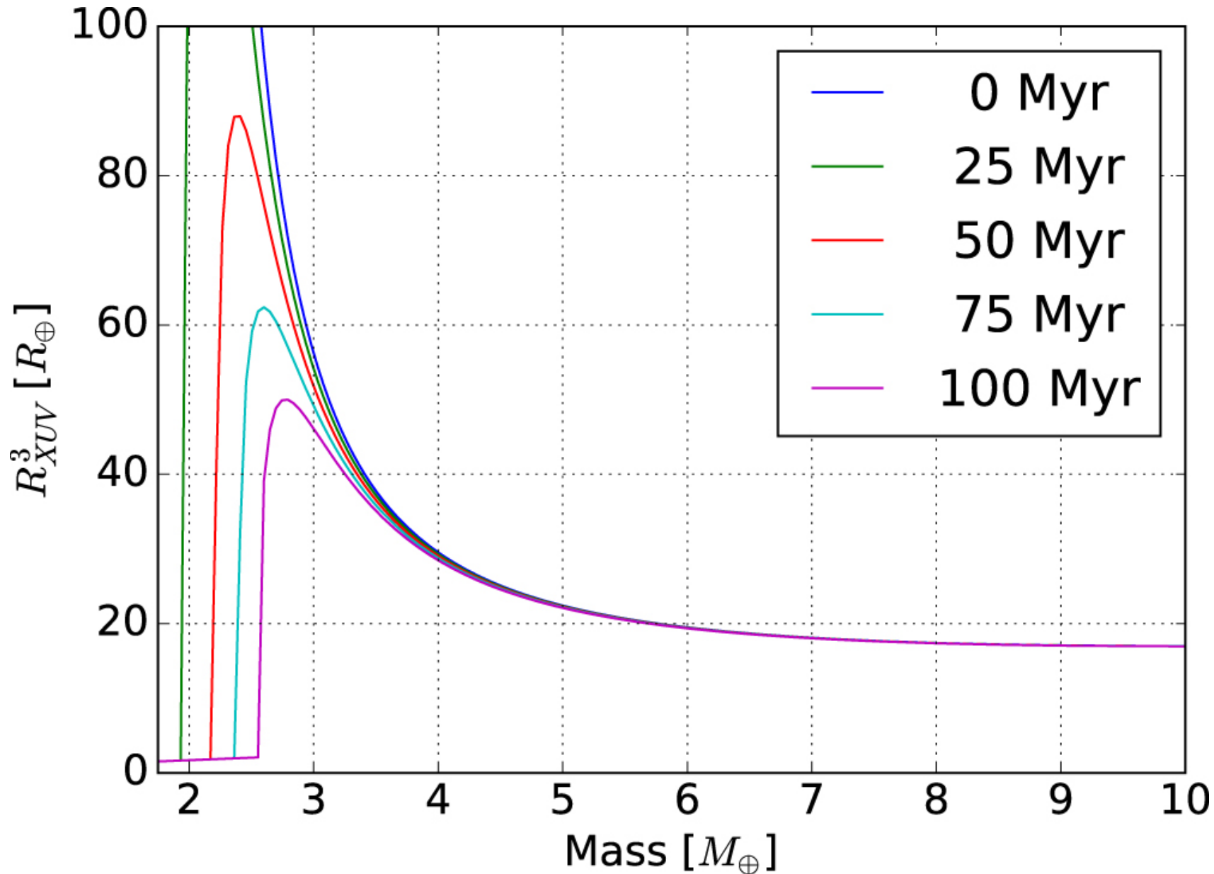
Figure 4. from Rocky Worlds Limited to 1.8 Earth Radii by Atmospheric Escape during a Star's Extreme UV Saturation null 2017 APJ 845 130 doi:10.3847/1538-4357/aa8137 https://dx.doi.org/10.3847/1538-4357/aa8137
