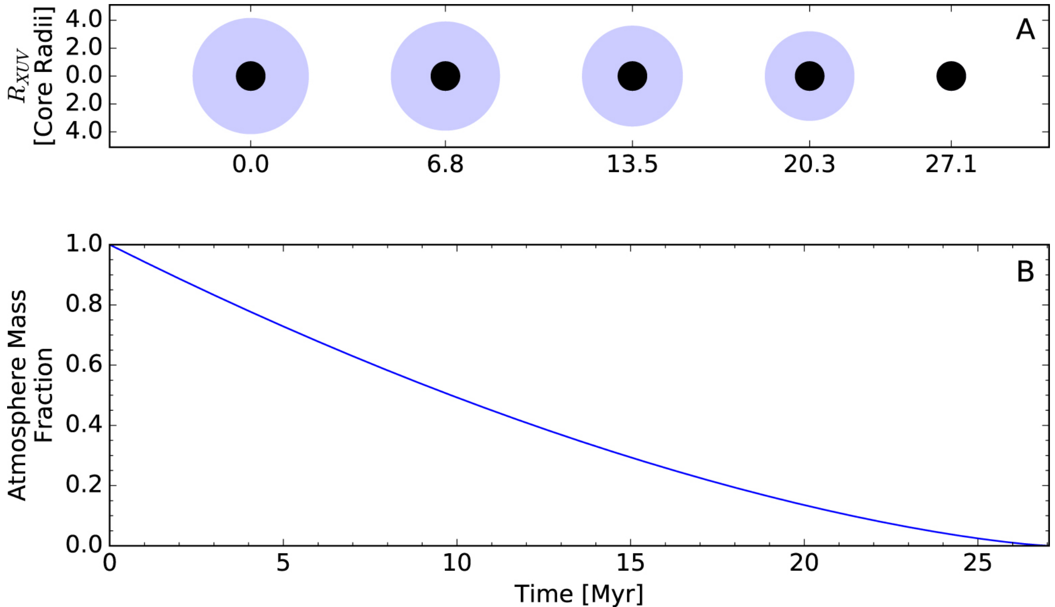
Figure 3. from Rocky Worlds Limited to 1.8 Earth Radii by Atmospheric Escape during a Star's Extreme UV Saturation null 2017 APJ 845 130 doi:10.3847/1538-4357/aa8137 https://dx.doi.org/10.3847/1538-4357/aa8137 © 2017. The American Astronomical Society. All rights reserved.
