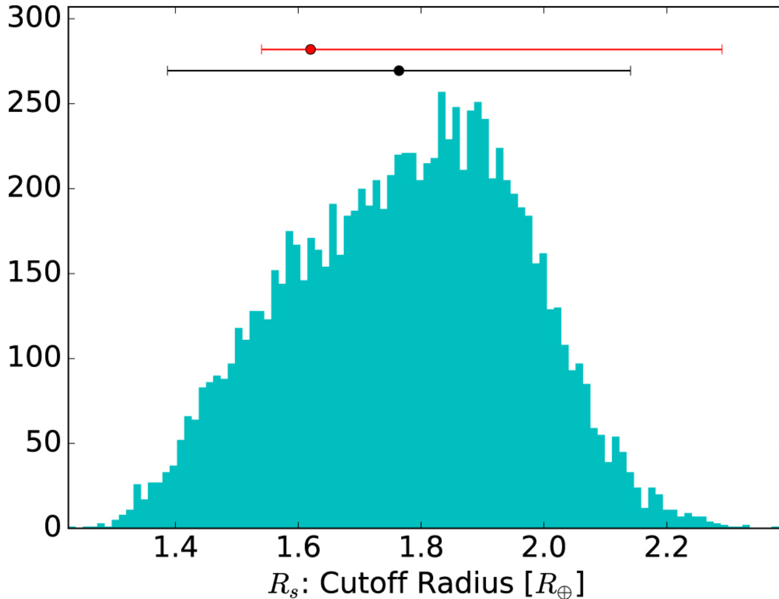
Figure 2. from Rocky Worlds Limited to 1.8 Earth Radii by Atmospheric Escape during a Star's Extreme UV Saturation null 2017 APJ 845 130 doi:10.3847/1538-4357/aa8137 https://dx.doi.org/10.3847/1538-4357/aa8137 © 2017. The American Astronomical Society. All rights reserved.
