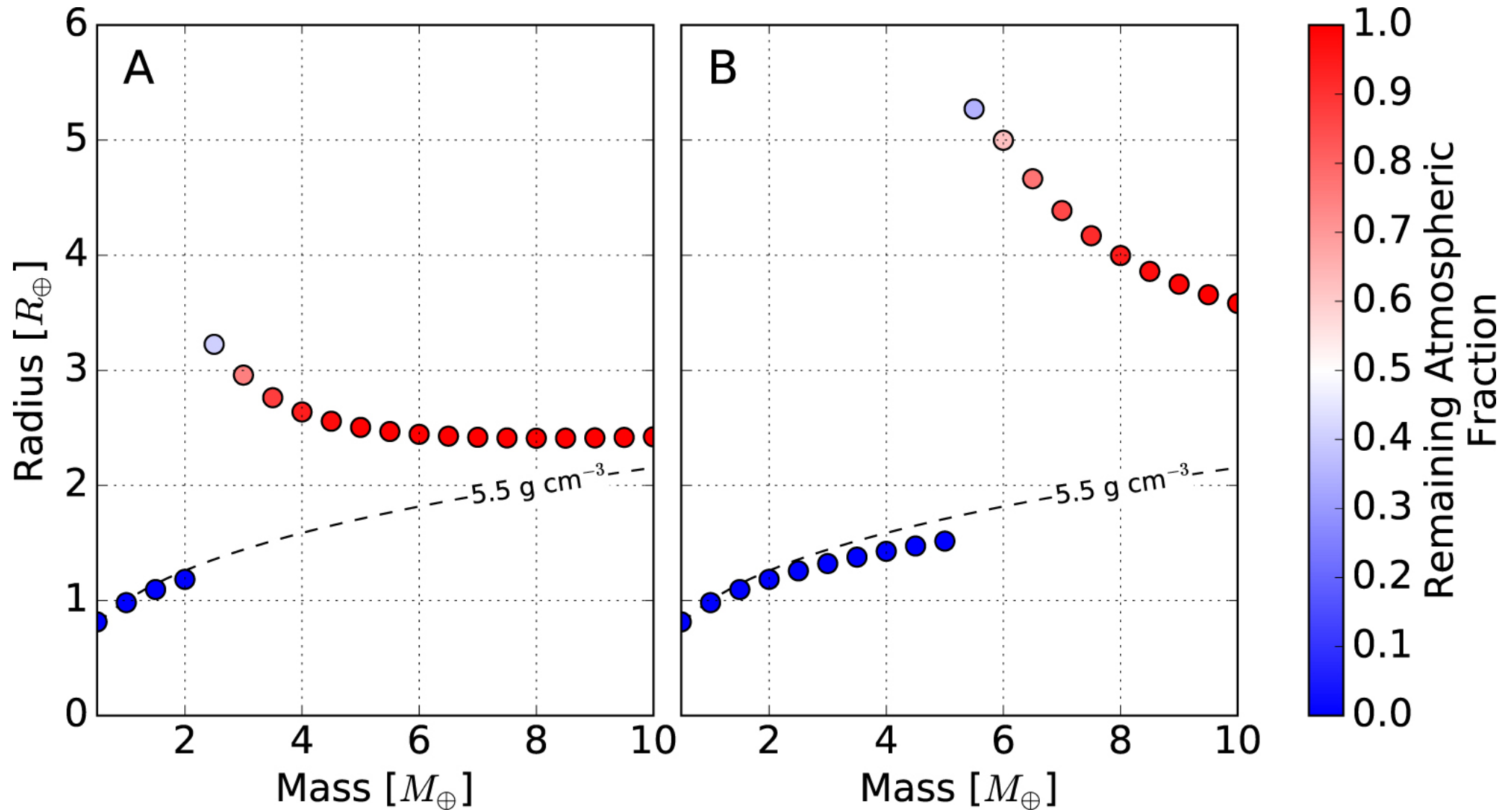
Figure 1. from Rocky Worlds Limited to 1.8 Earth Radii by Atmospheric Escape during a Star's Extreme UV Saturation null 2017 APJ 845 130 doi:10.3847/1538-4357/aa8137 https://dx.doi.org/10.3847/1538-4357/aa8137
