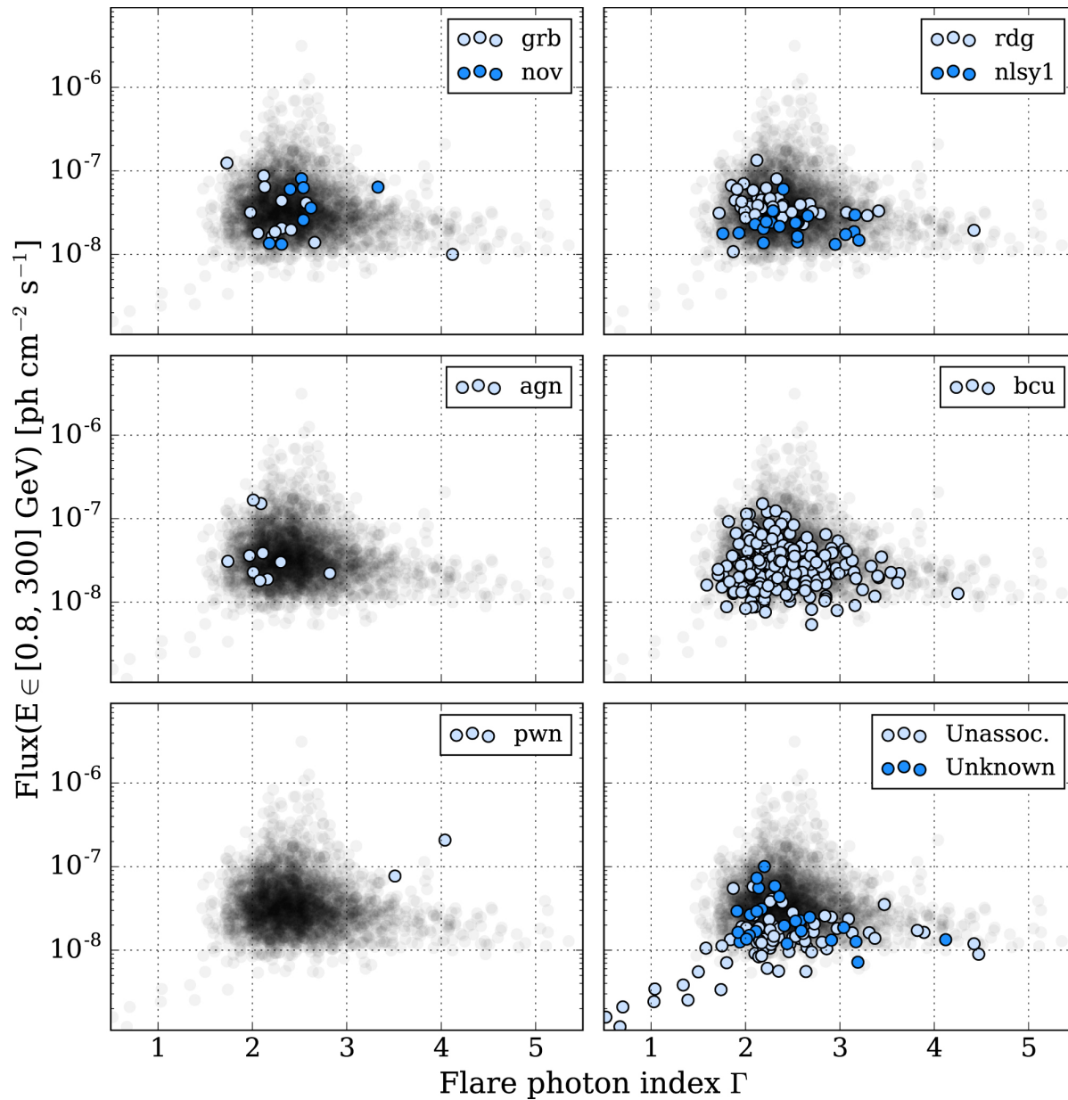
Figure 9. from The Second Catalog of Flaring Gamma-Ray Sources from the Fermi All-sky Variability Analysis null 2017 APJ 846 34 doi:10.3847/1538-4357/aa8092 https://dx.doi.org/10.3847/1538-4357/aa8092 © 2017. The American Astronomical Society. All rights reserved.
