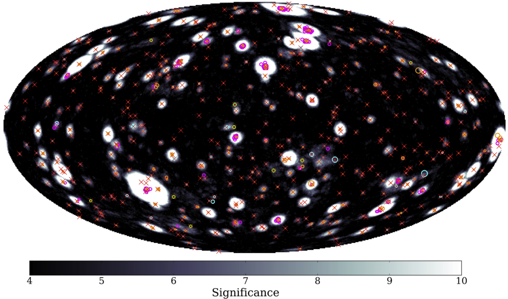
Figure 5. from The Second Catalog of Flaring Gamma-Ray Sources from the Fermi All-sky Variability Analysis null 2017 APJ 846 34 doi:10.3847/1538-4357/aa8092 https://dx.doi.org/10.3847/1538-4357/aa8092 © 2017. The American Astronomical Society. All rights reserved.
