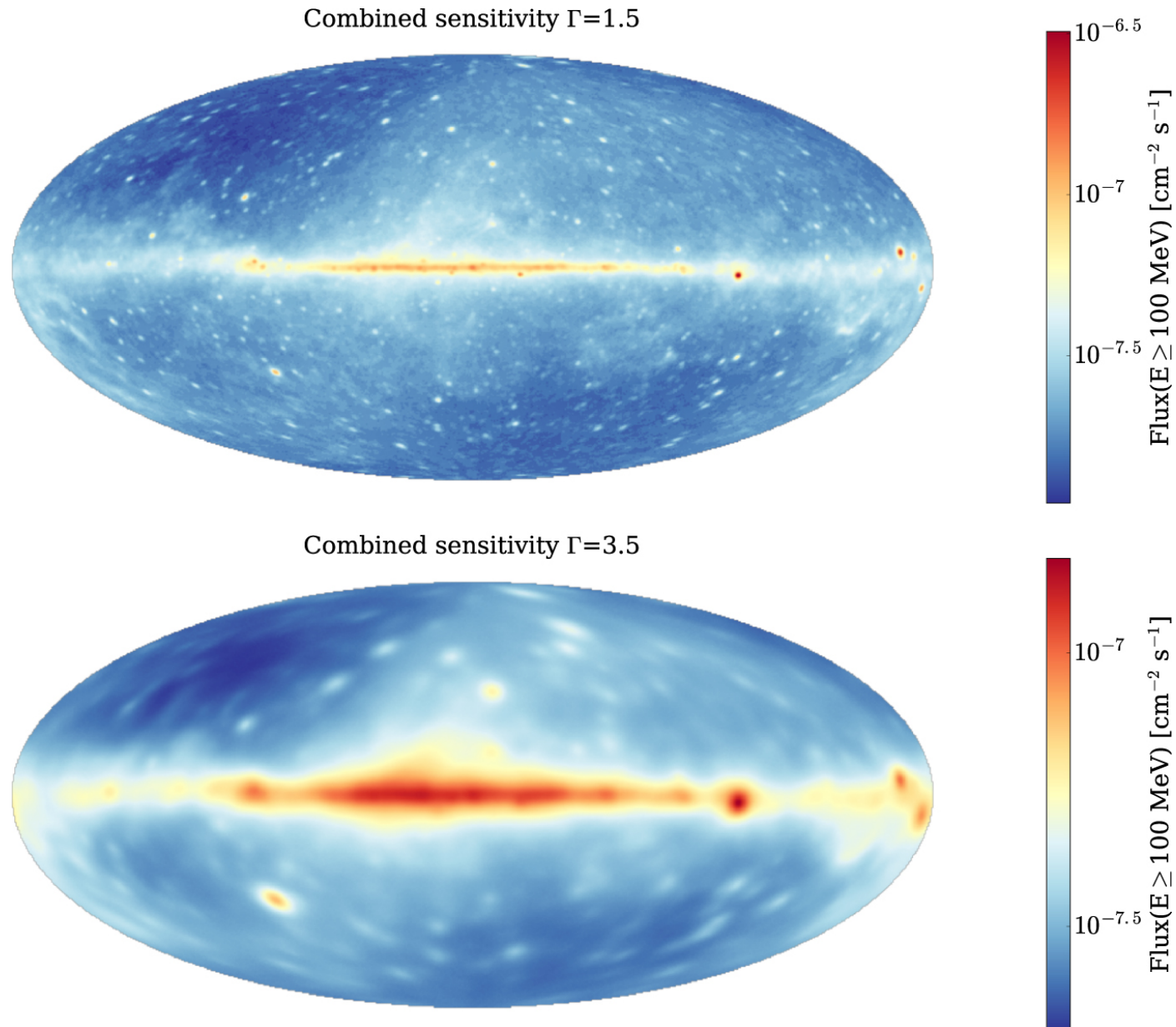
Figure 4. from The Second Catalog of Flaring Gamma-Ray Sources from the Fermi All-sky Variability Analysis null 2017 APJ 846 34 doi:10.3847/1538-4357/aa8092 https://dx.doi.org/10.3847/1538-4357/aa8092 © 2017. The American Astronomical Society. All rights reserved.
