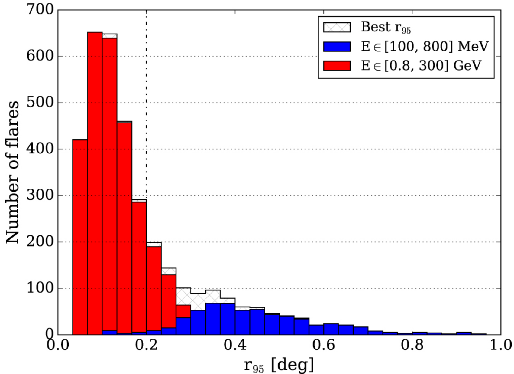
Figure 3. from The Second Catalog of Flaring Gamma-Ray Sources from the Fermi All-sky Variability Analysis null 2017 APJ 846 34 doi:10.3847/1538-4357/aa8092 https://dx.doi.org/10.3847/1538-4357/aa8092 © 2017. The American Astronomical Society. All rights reserved.
