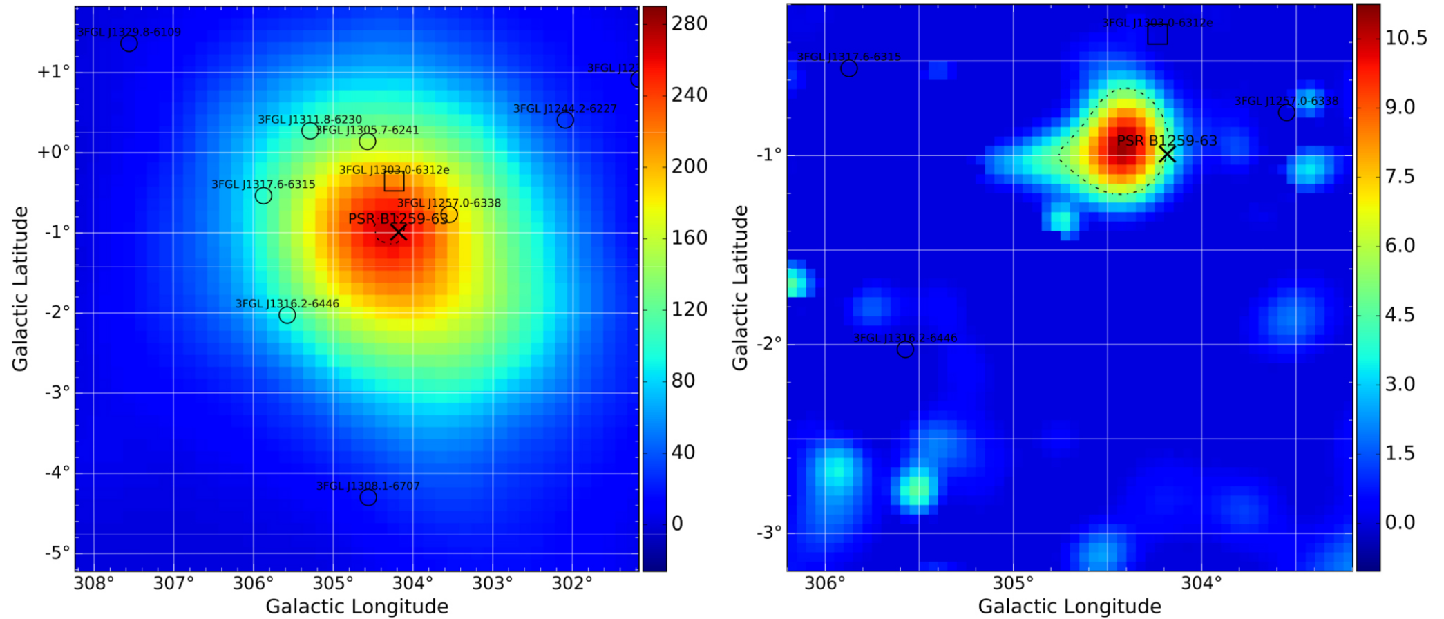
Figure 2. from The Second Catalog of Flaring Gamma-Ray Sources from the Fermi All-sky Variability Analysis null 2017 APJ 846 34 doi:10.3847/1538-4357/aa8092 https://dx.doi.org/10.3847/1538-4357/aa8092 © 2017. The American Astronomical Society. All rights reserved.
