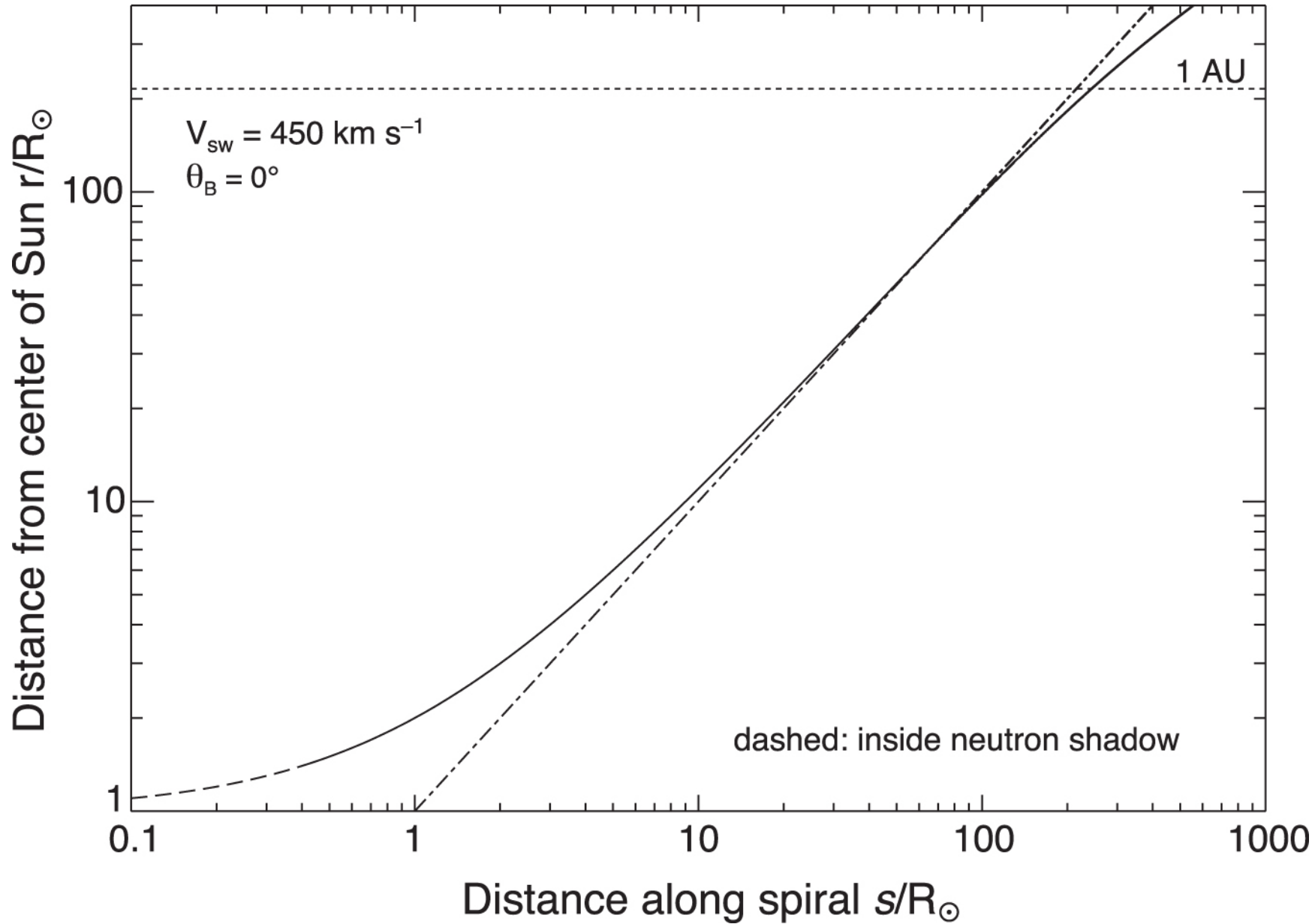
Figure 9. from Neutron-decay Protons from Solar Flares as Seed Particles for CME-shock Acceleration in the Inner Heliosphere null 2017 APJ 846 53 doi:10.3847/1538-4357/aa7fb3 https://dx.doi.org/10.3847/1538-4357/aa7fb3 © 2017. The American Astronomical Society. All rights reserved.
