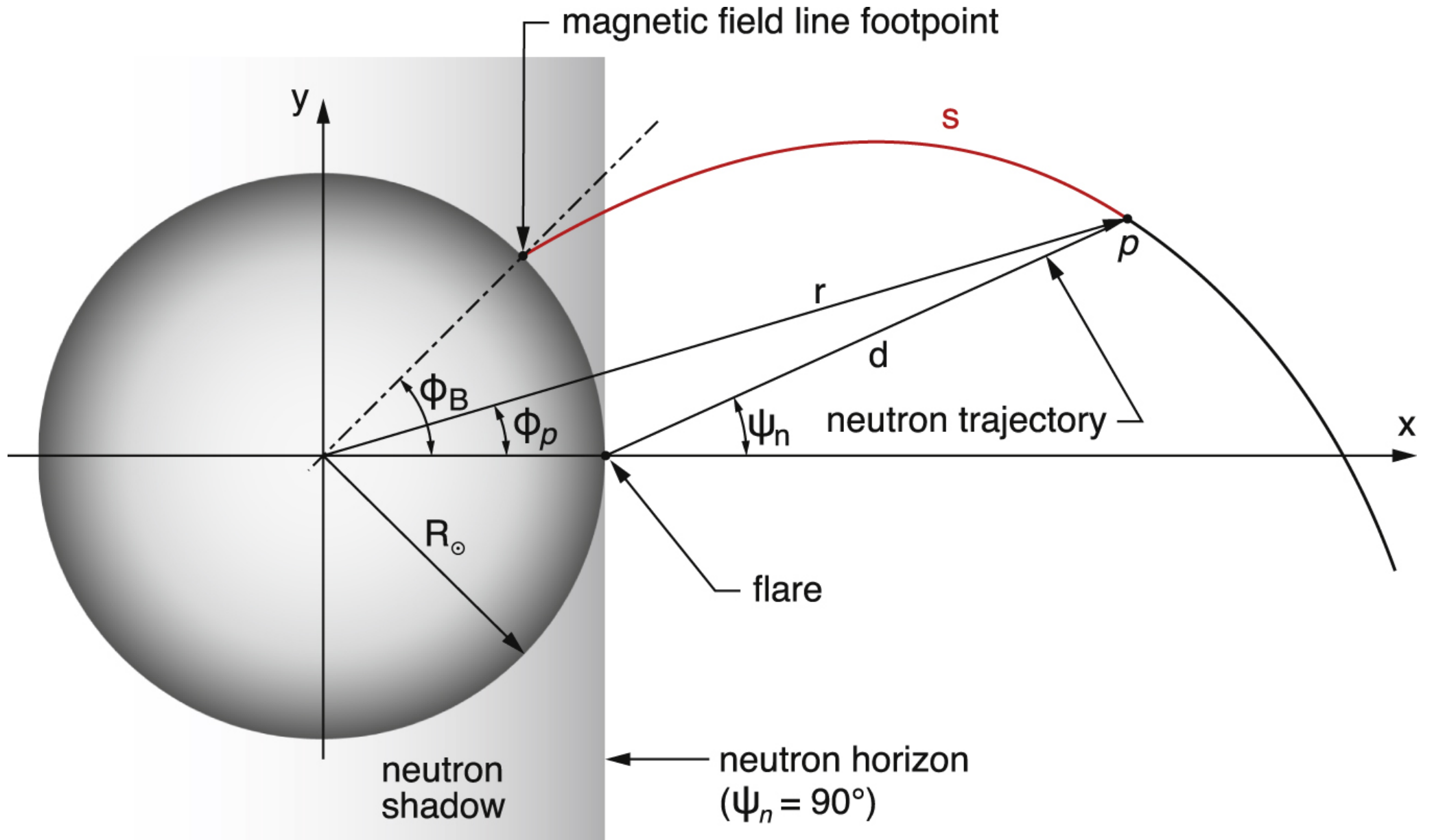
Figure 8. from Neutron-decay Protons from Solar Flares as Seed Particles for CME-shock Acceleration in the Inner Heliosphere null 2017 APJ 846 53 doi:10.3847/1538-4357/aa7fb3 https://dx.doi.org/10.3847/1538-4357/aa7fb3 © 2017. The American Astronomical Society. All rights reserved.
